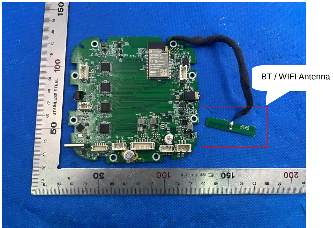
INTERNAL VIEW OF EUT (FIGURE 9)
