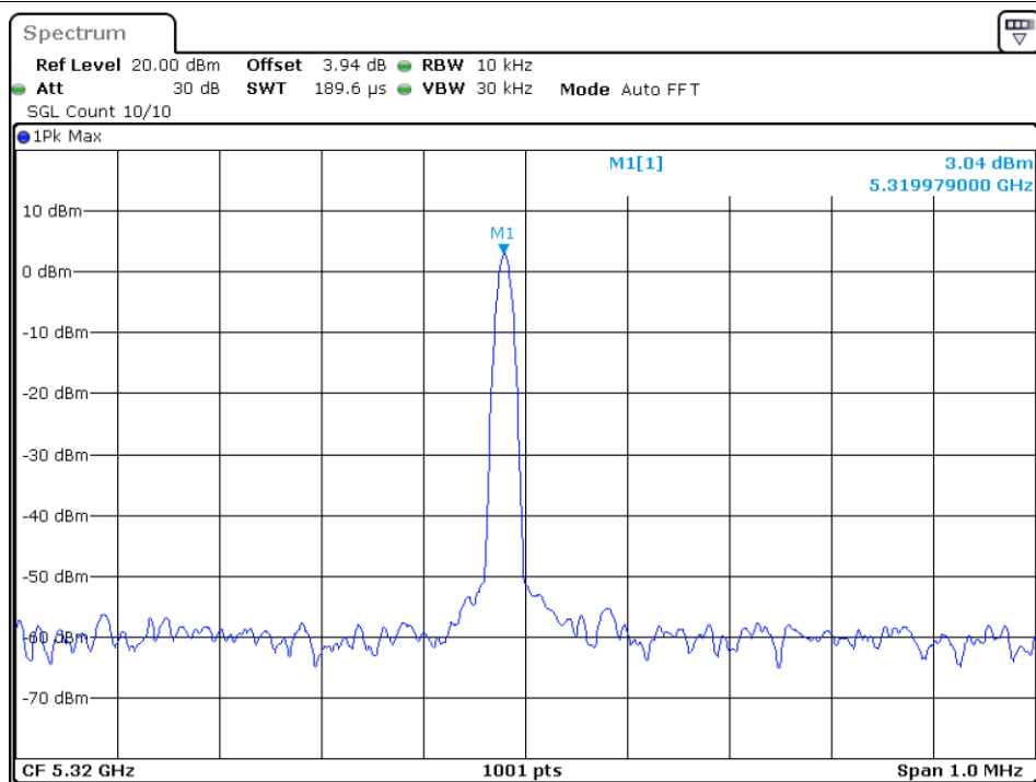
Freq. Stability 30C 120V ac20 5320MHz Ant1
