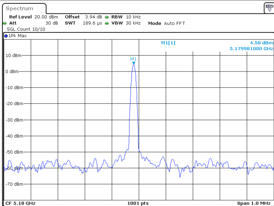
Freq. Stability 20C 120V ax20 5180MHz Ant1
