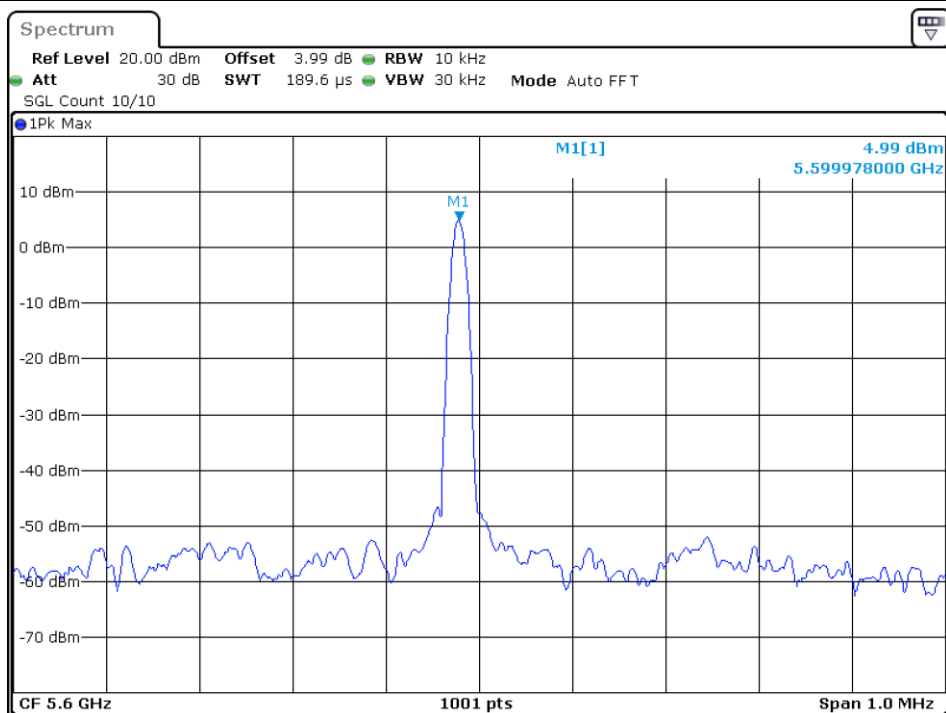
Freq. Stability 10C 120V ax20 5600MHz Ant1
