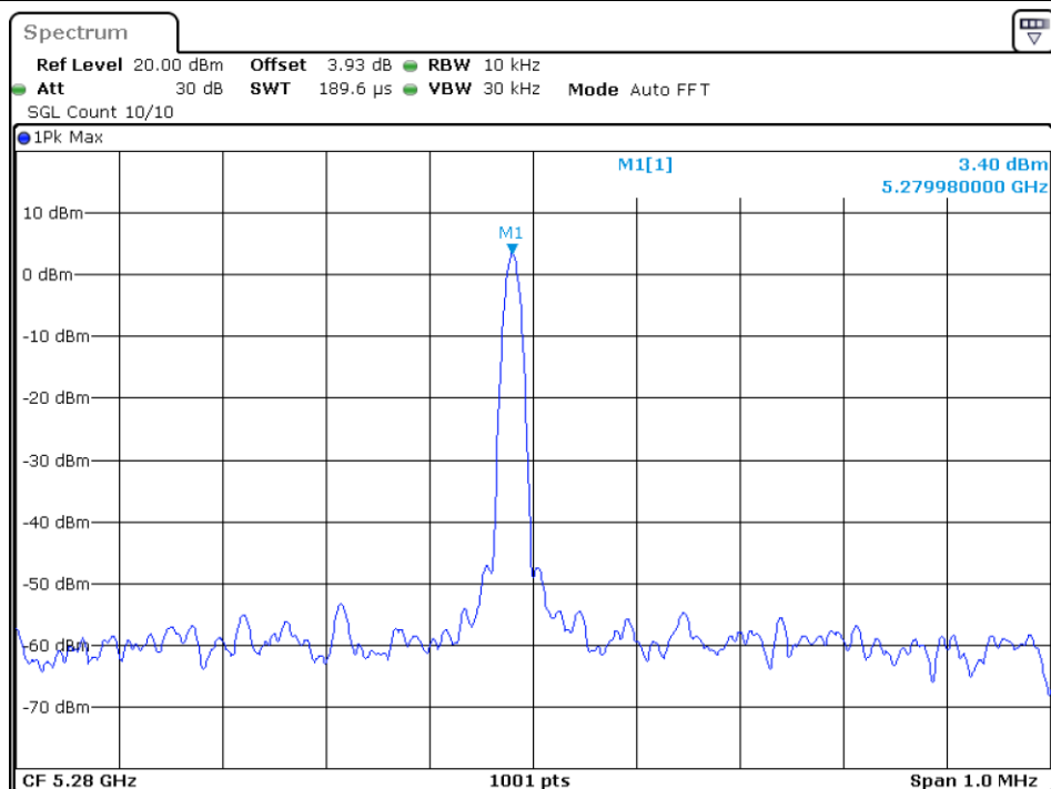
Freq. Stability 0C 120V ac20 5280MHz Ant1
