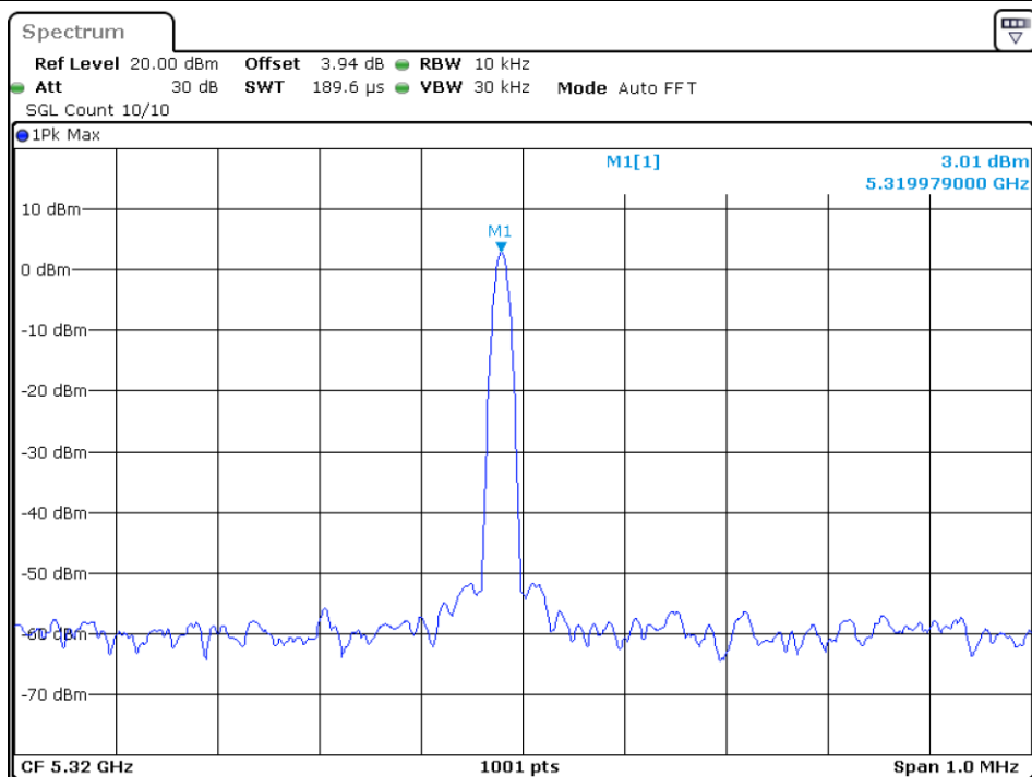
Freq. Stability 30C 120V ax20 5320MHz Ant1
