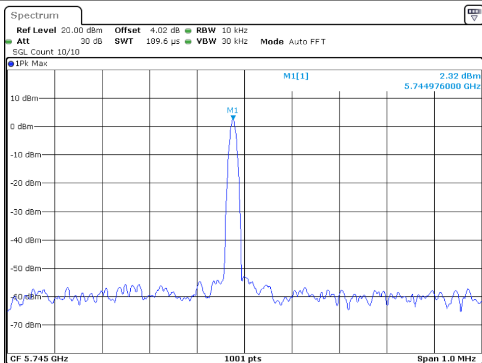
Freq. Stability 10C 120V ac20 5745MHz Ant1
