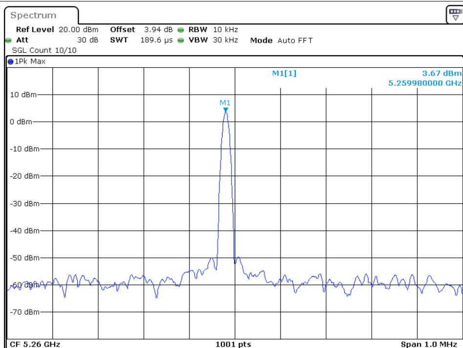
Freq. Stability 10C 120V ac20 5260MHz Ant1
