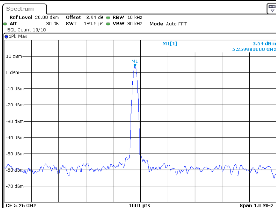
Freq. Stability 10C 120V ax20 5260MHz Ant1
