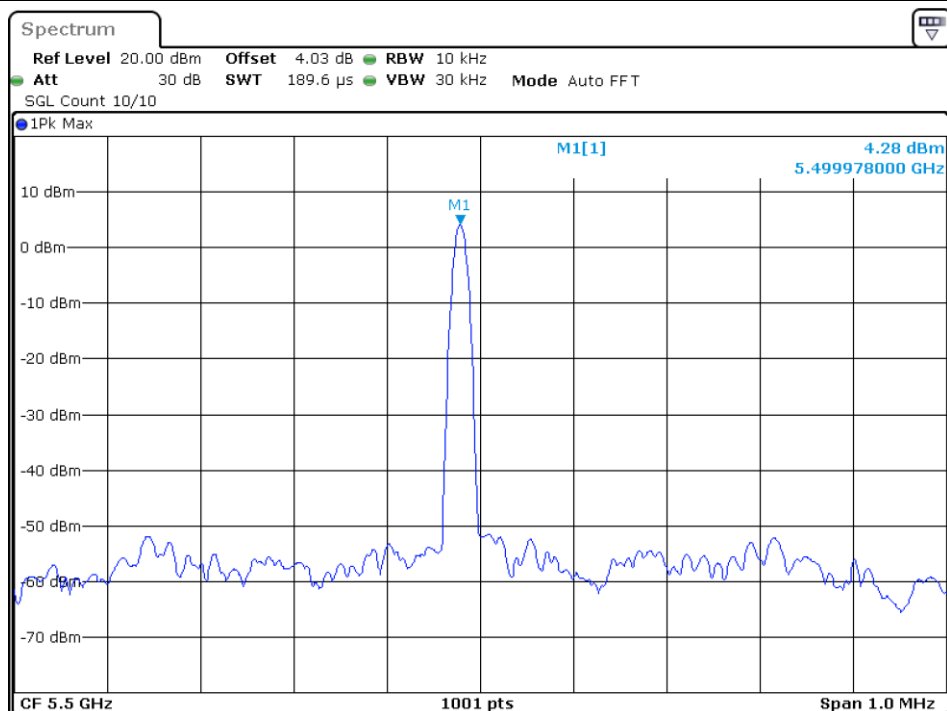
Freq. Stability 20C 120V ax20 5500MHz Ant1
