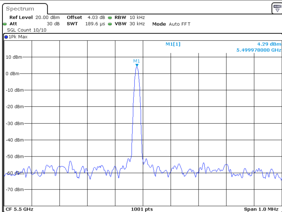
Freq. Stability 40C 120V ax20 5500MHz Ant1
