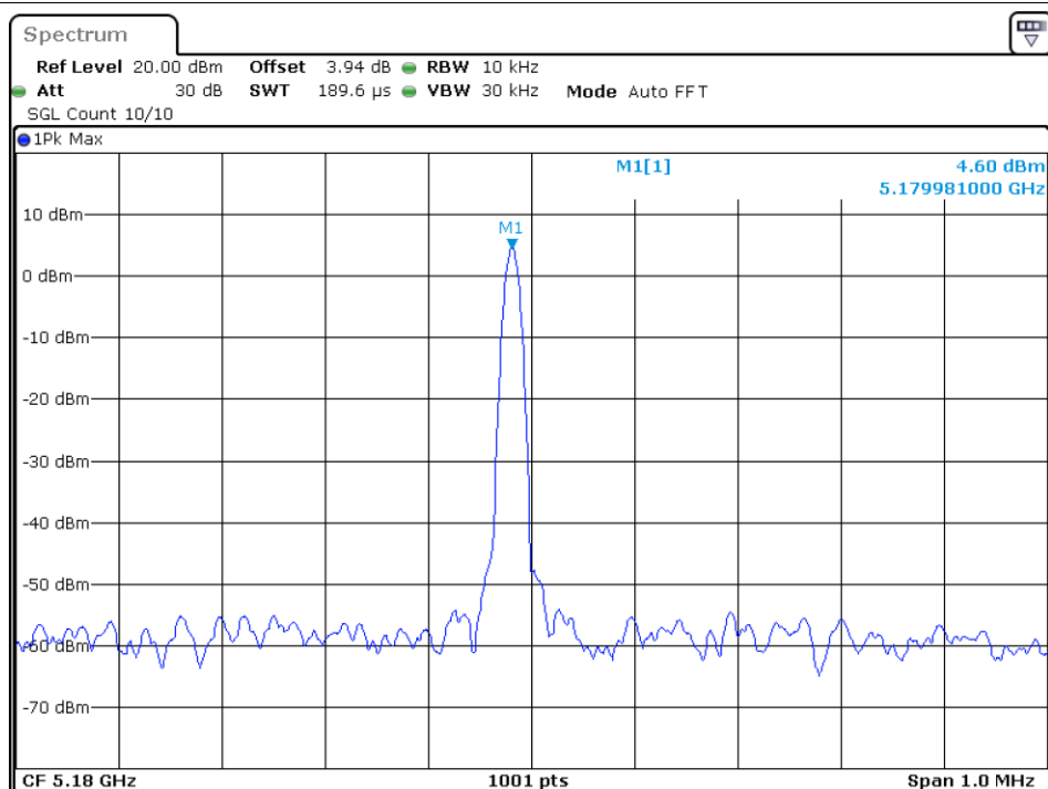
Freq. Stability 40C 120V ac20 5180MHz Ant1
