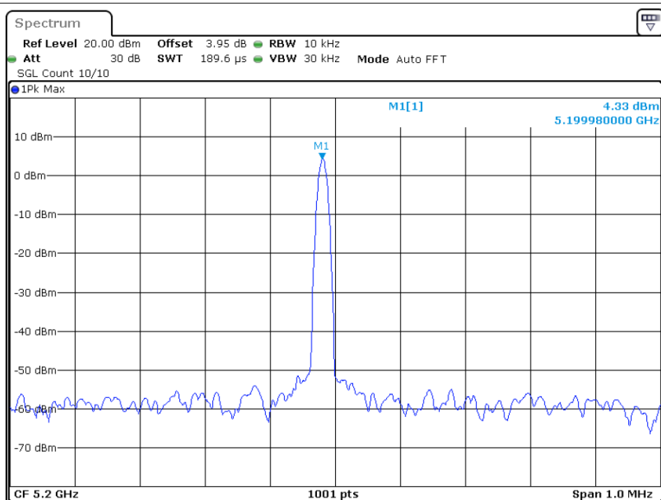
Freq. Stability 10C 120V ax20 5200MHz Ant1
