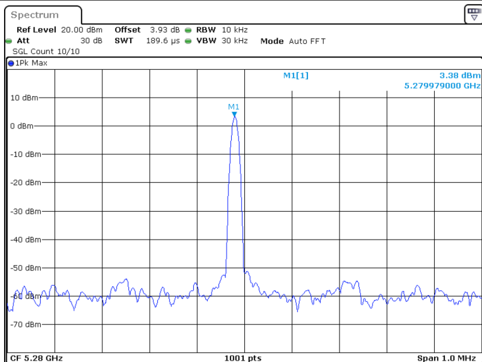
Freq. Stability 20C 120V ax20 5280MHz Ant1
