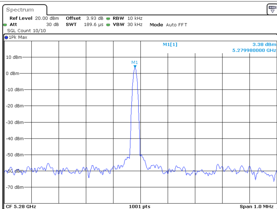
Freq. Stability 20C 120V ac20 5280MHz Ant1
