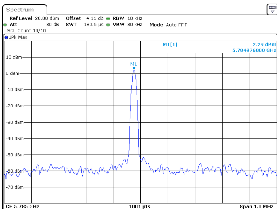
Freq. Stability 20C 120V ac20 5785MHz Ant1
