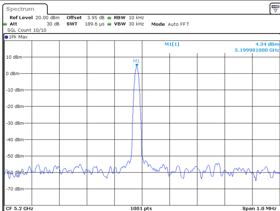
Freq. Stability 10C 120V ac20 5200MHz Ant1
