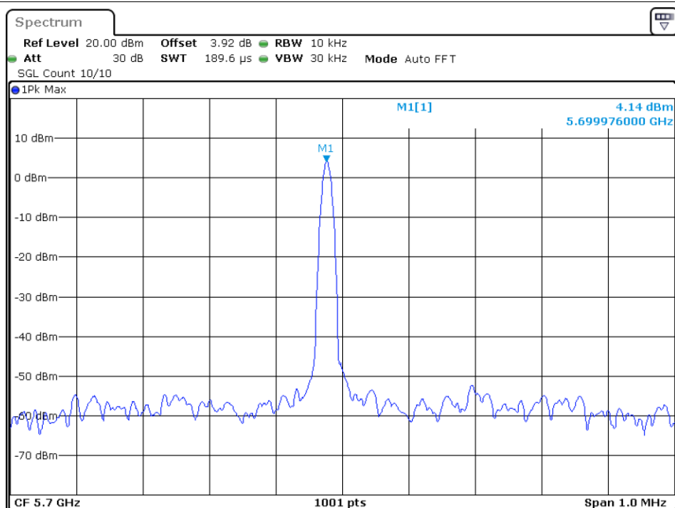
Freq. Stability 0C 120V ac20 5700MHz Ant1
