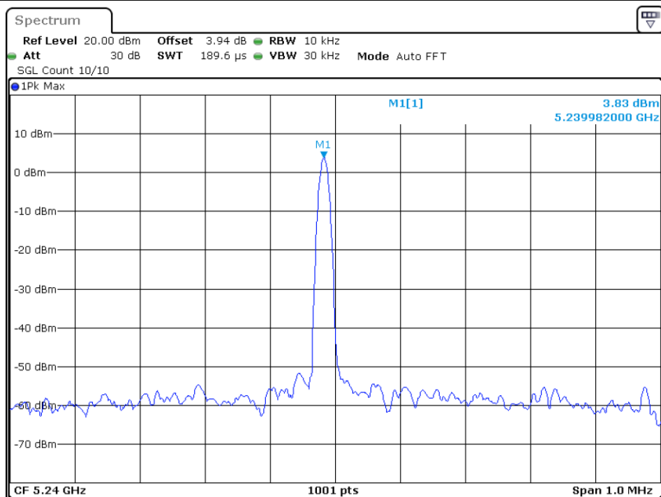
Freq. Stability 20C 120V ax20 5240MHz Ant1
