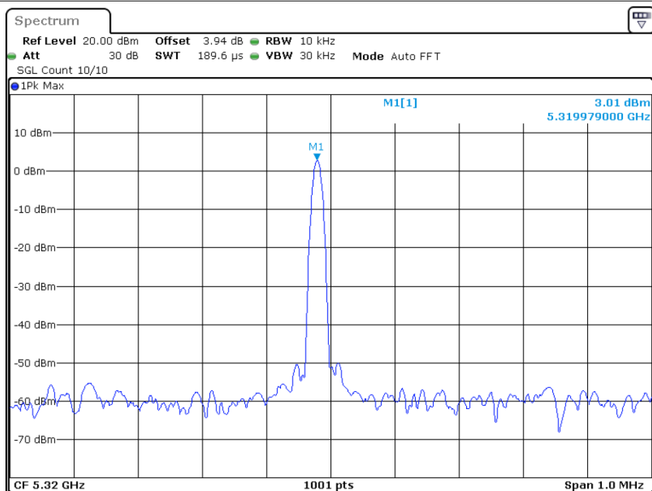
Freq. Stability 10C 120V ax20 5320MHz Ant1
