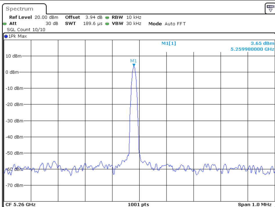
Freq. Stability 30C 120V ac20 5260MHz Ant1
