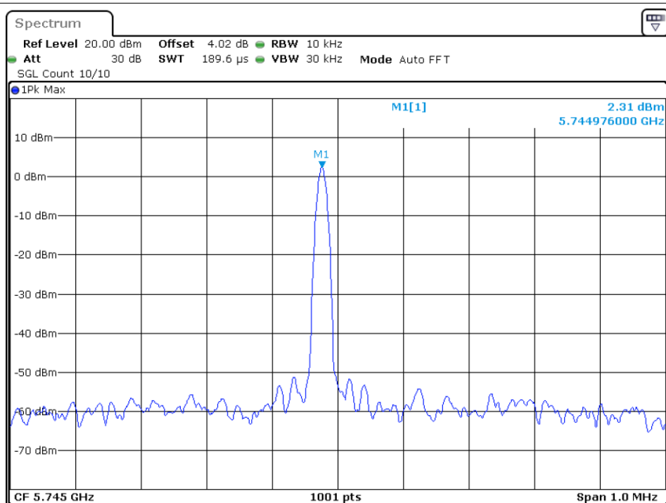
Freq. Stability 30C 120V ac20 5745MHz Ant1
