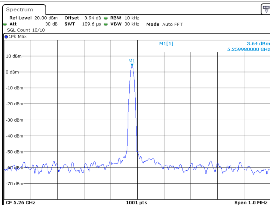
Freq. Stability 30C 120V ax20 5260MHz Ant1
