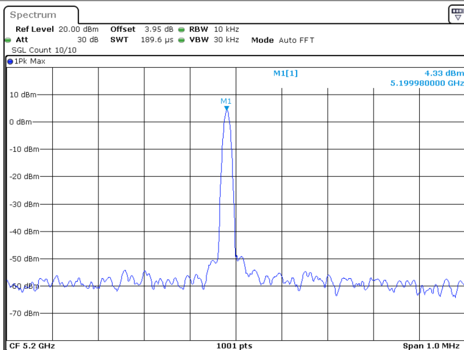
Freq. Stability 30C 120V ax20 5200MHz Ant1
