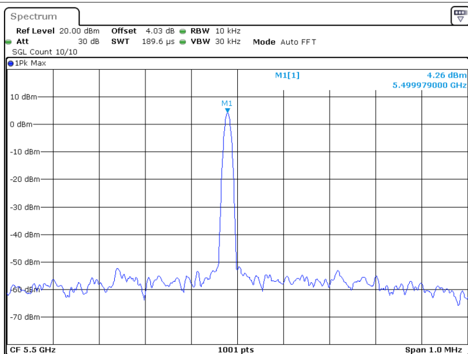
Freq. Stability 0C 120V ac20 5500MHz Ant1
