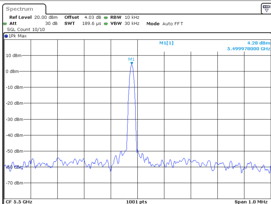
Freq. Stability 0C 120V ax20 5500MHz Ant1
