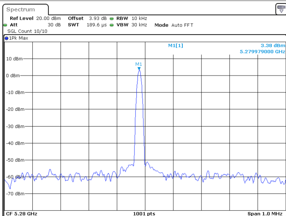
Freq. Stability 0C 120V ax20 5280MHz Ant1
