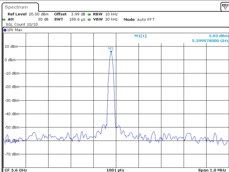
Freq. Stability 10C 120V ac20 5600MHz Ant1
