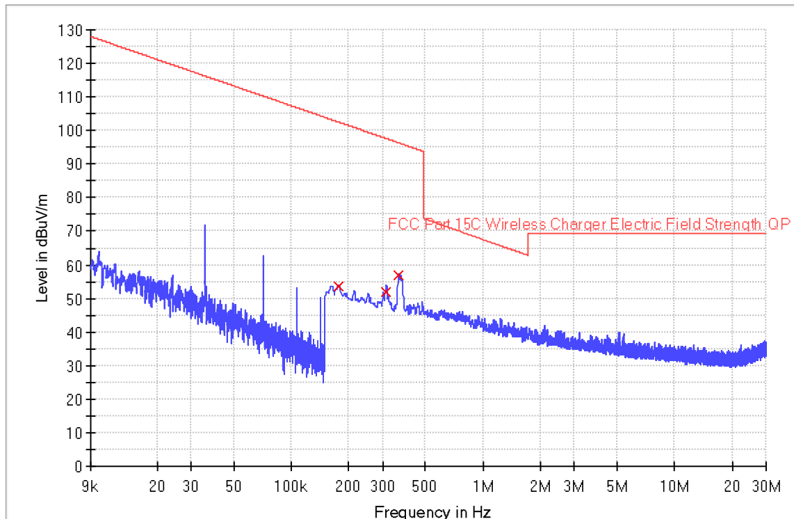
FCC Part 9K-30M(dBuV)
