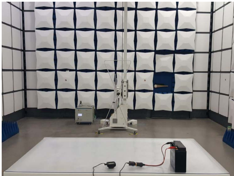
Radiated Emission
