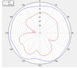
Phi=90 freq=2490MHz
