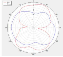
Phi=0 freq=2470MHz
