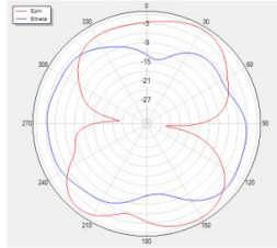
Phi=0 freq=2500MHz
