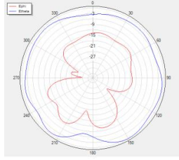
Phi=90 freq=2470MHz
