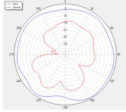
Phi=90 freq=2480MHz
