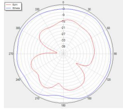
Phi=90 freq=2500MHz
