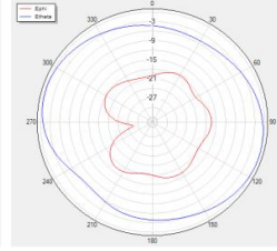
Theta=90 freq=2480MHz
