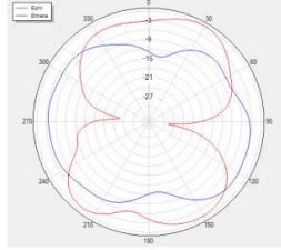
Phi=0 freq=2490MHz
