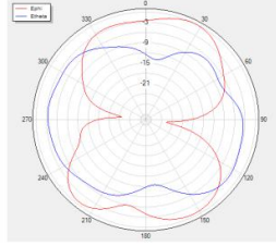
Phi=0 freq=2480MHz
