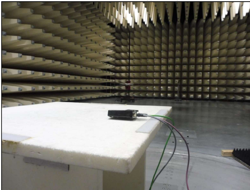
Photo 1: Radiated Emission 30MHz - 1GHz
