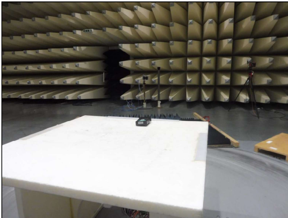
Photo 2: Radiated Emission 1GHz - 10GHz
