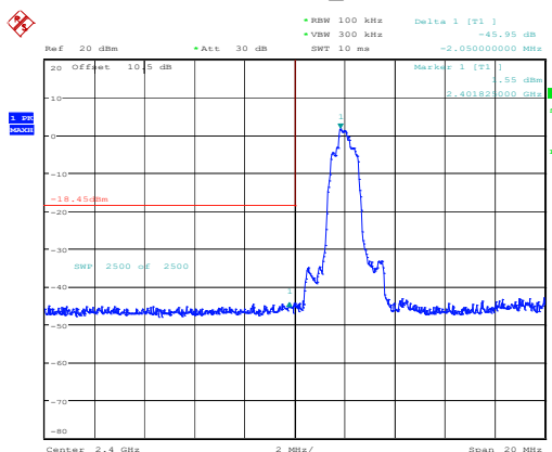
3DH1_Low
