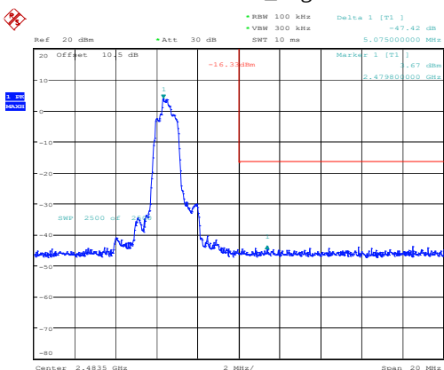
3DH1_High
