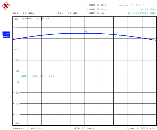
DH1_High
