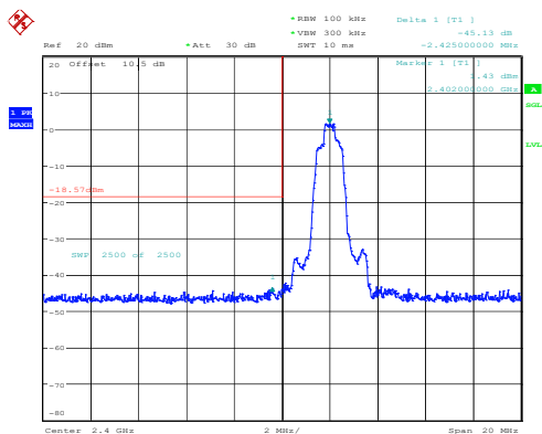
2DH1_Low
