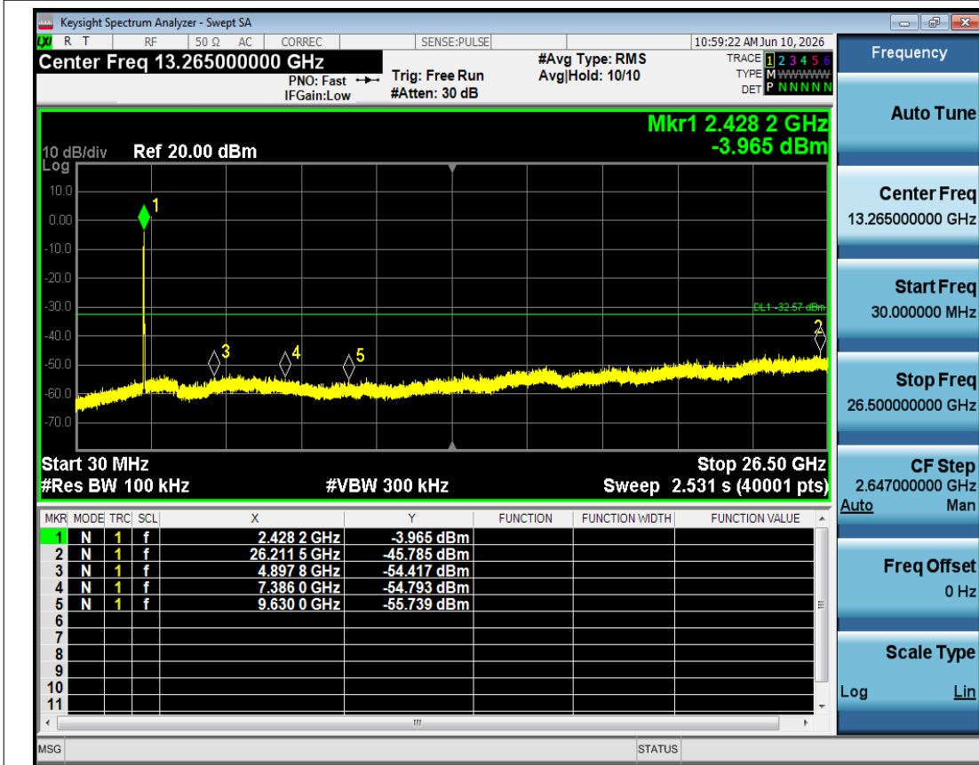
Tx. Spurious NVNT ax40 2422MHz Ant1 Emission
