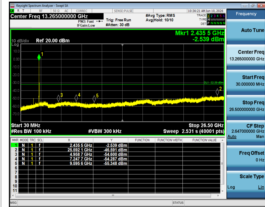
Tx. Spurious NVNT ax20 2437MHz Ant1 Emission
