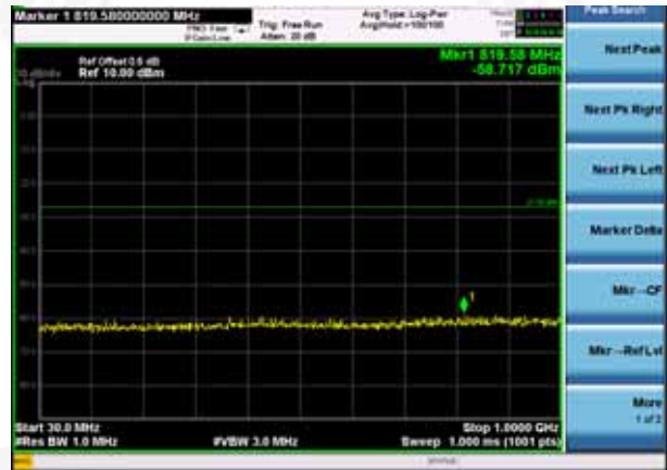
802.11 ac80 on channel 155
