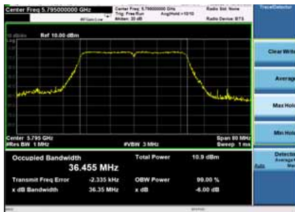
(802.11 n40) 99%Bandwidth plot on channel 159
