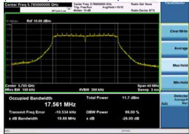
(802.11 n20) -26dB Bandwidth plot on channel 157
