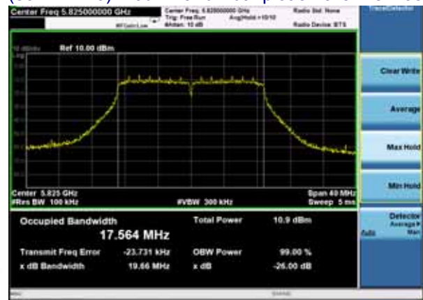
(802.11 n20) -26dB Bandwidth plot on channel 165
