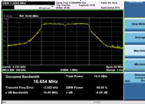
(802.11a) 99%Bandwidth plot on channel 149
