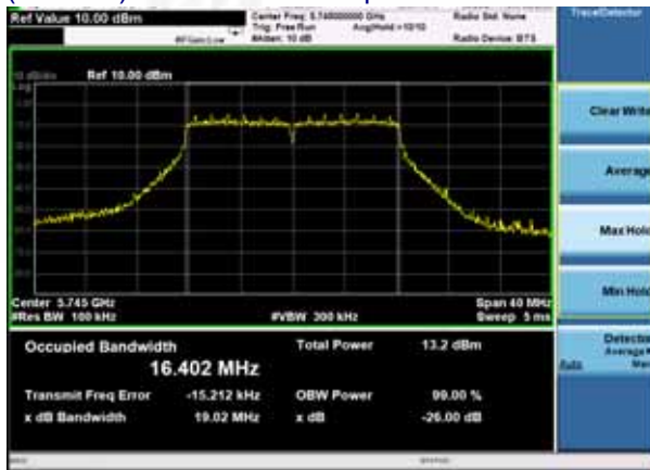
(802.11a) -26dB Bandwidth plot on channel 149
