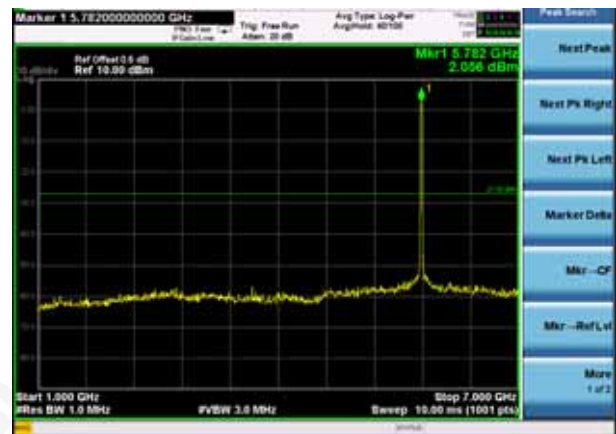
802.11a on channel 157
