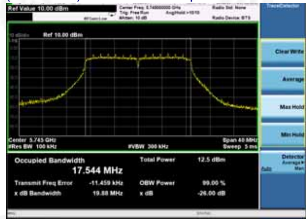
(802.11 n20) -26dB Bandwidth plot on channel 149
