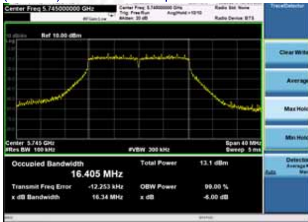
(802.11a) -6dB Bandwidth plot on channel 149
