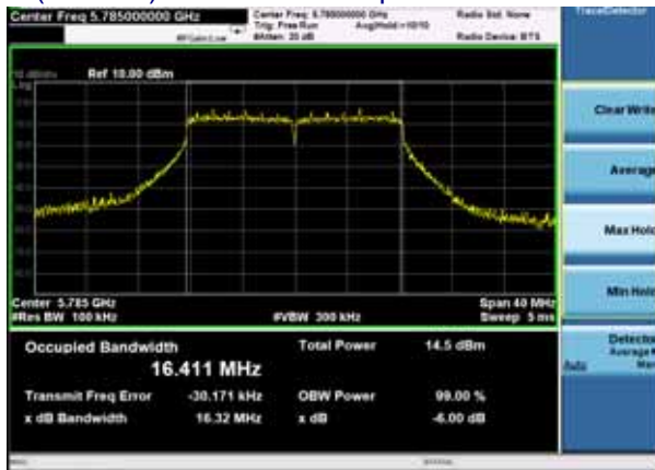
(802.11a) -6dB Bandwidth plot on channel 157
