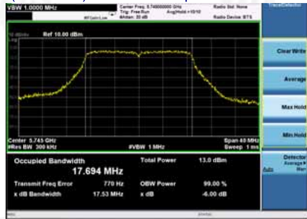
(802.11 n20) 99%Bandwidth plot on channel 149
