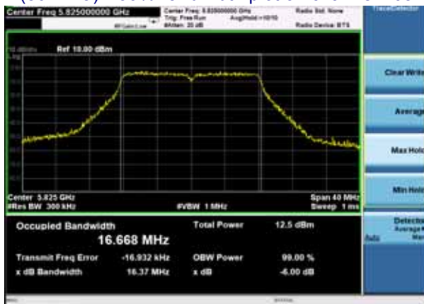
(802.11a) 99%Bandwidth plot on channel 165
