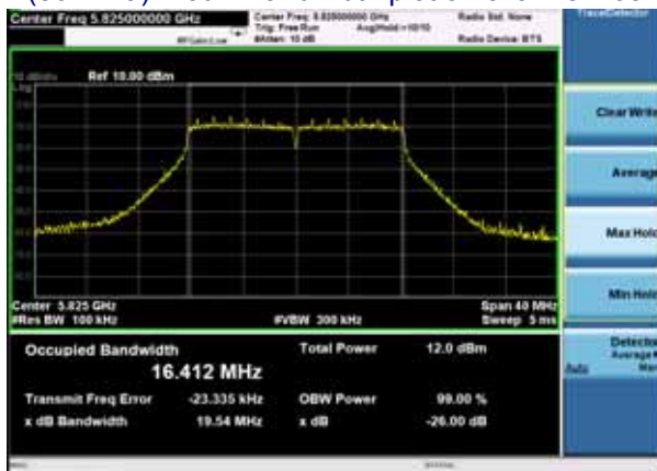
(802.11a) -26dB Bandwidth plot on channel 165
