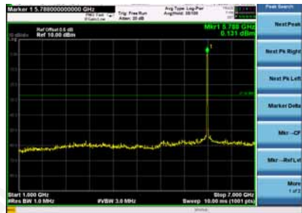
802.11ac20 on channel 157
