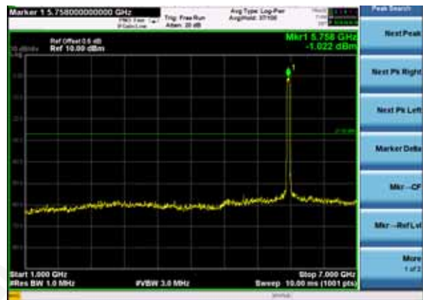
802.11ac40 on channel 151
