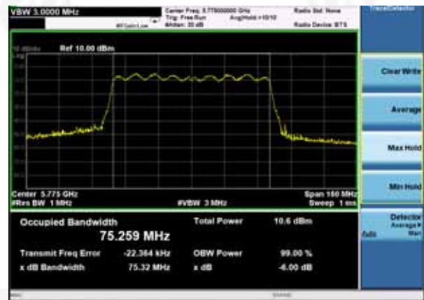
(802.11 AC80) 99%Bandwidth plot on channel 155
