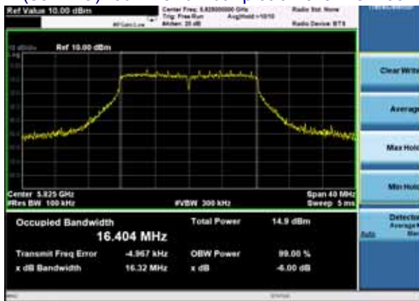
(802.11a) -6dB Bandwidth plot on channel 165
