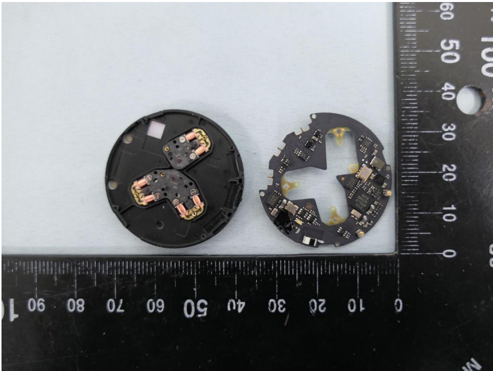
(6) EUT Photo - Plastic
