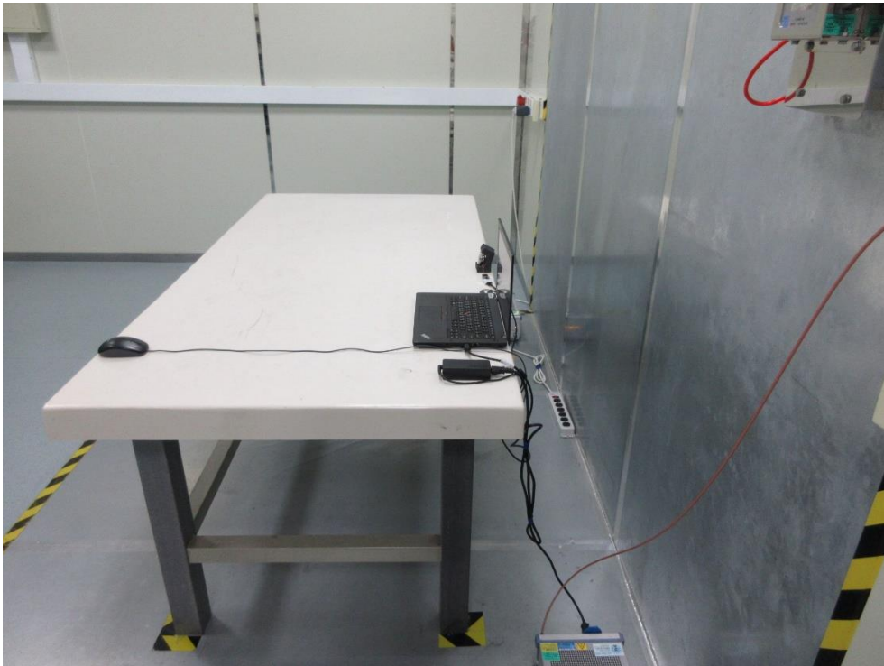
Description: Back View of Conducted Emission Test Setup - Titanium
