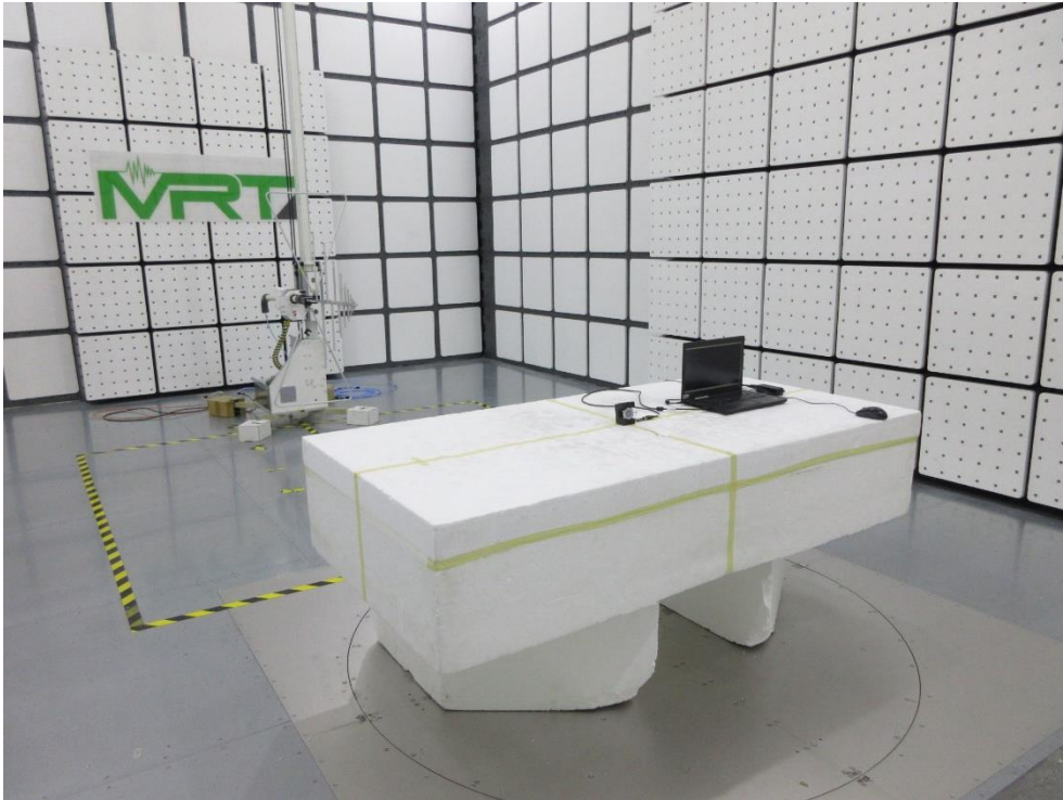
Description: Radiated Emission Test Setup for above 1GHz - Titanium
