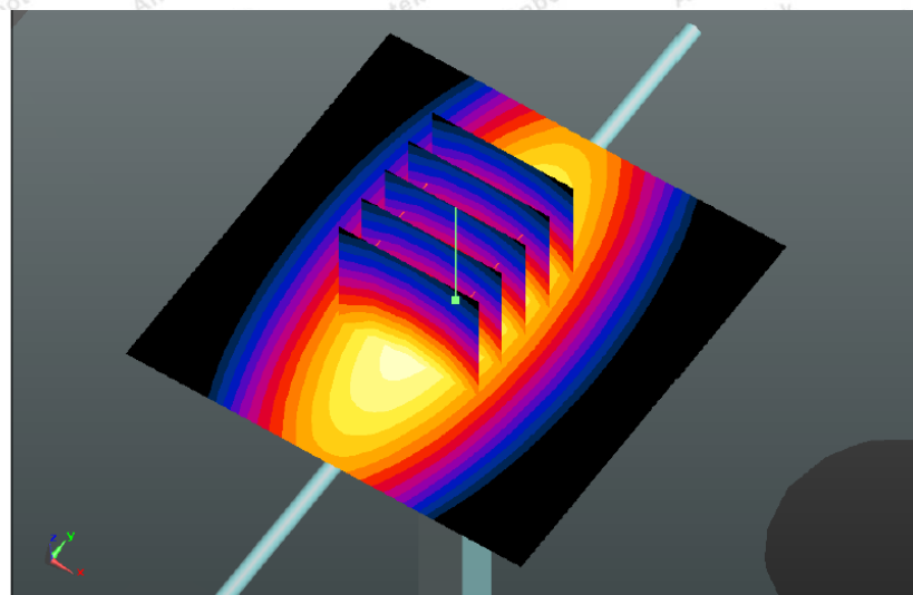
System Performance Check 835MHz Body 250mW
