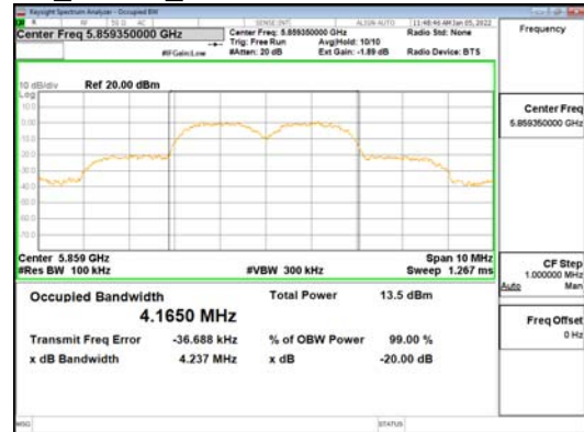
ANT1_Digital Modulation_4MHz_BW
