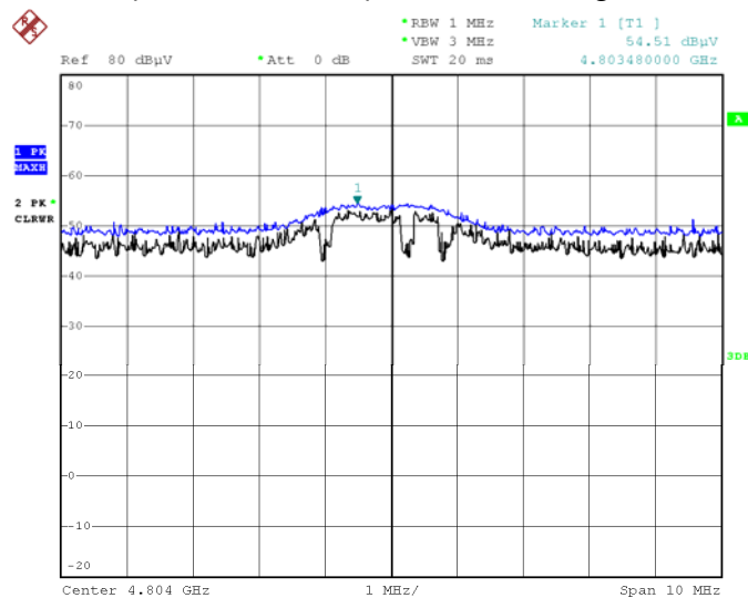
Radiated Spurious Emissions plot – Peak Reading (Ch.0 2nd Harmonic)
