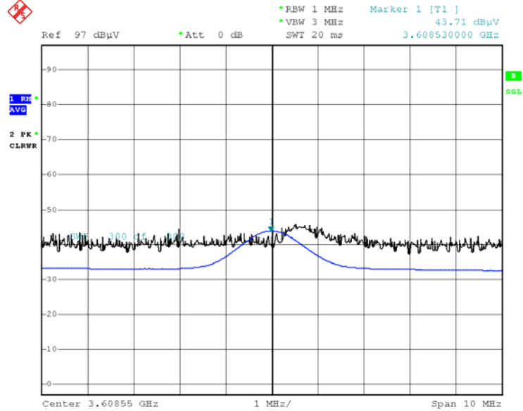
Radiated Spurious Emissions plot –Average Reading (RC2 4th Harmonic)
