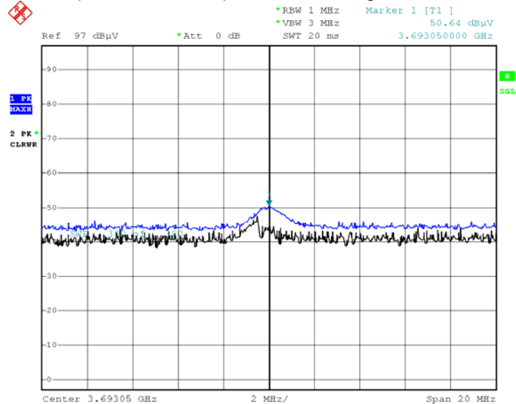
Radiated Spurious Emissions plot – Peak Reading (RC4 4th Harmonic)
