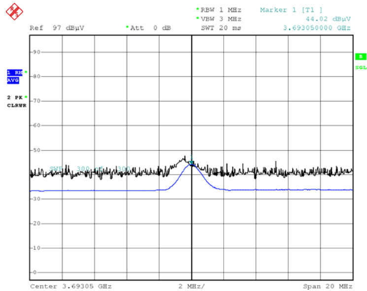
Radiated Spurious Emissions plot –Average Reading (RC4 4th Harmonic)
