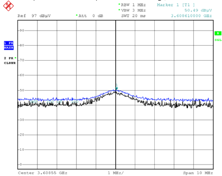
Radiated Spurious Emissions plot – Peak Reading (RC2 4th Harmonic)
