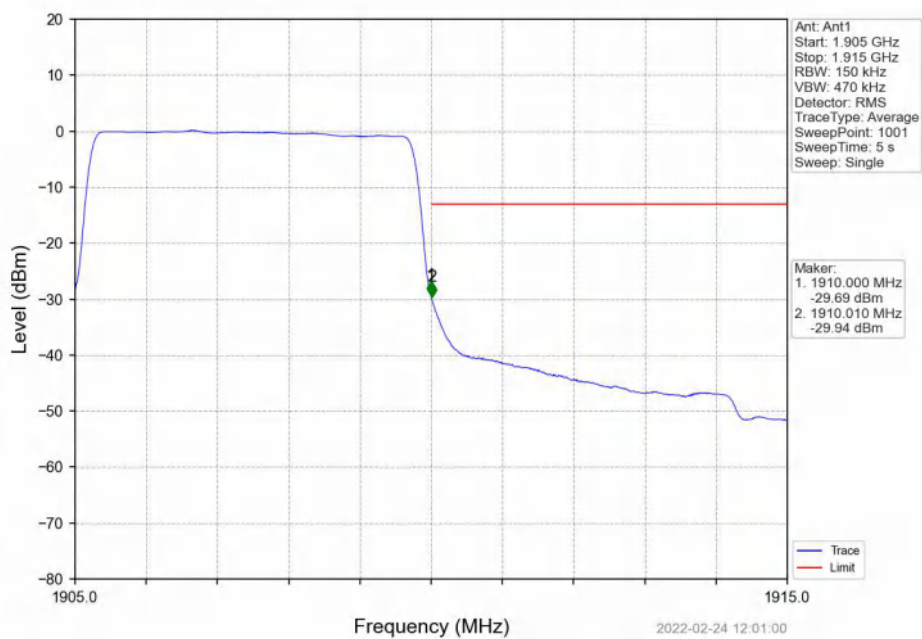
Band2_5MHz_QPSK_HCH_1907.5MHz_RB_25_0_NTNV
