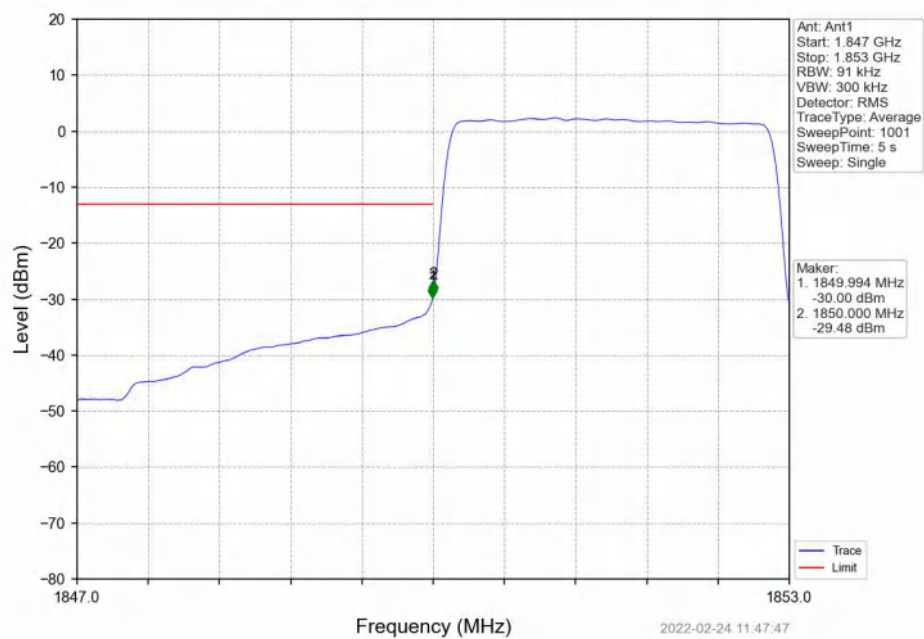
Band2_3MHz_QPSK_LCH_1851.5MHz_RB_15_0_NTNV
