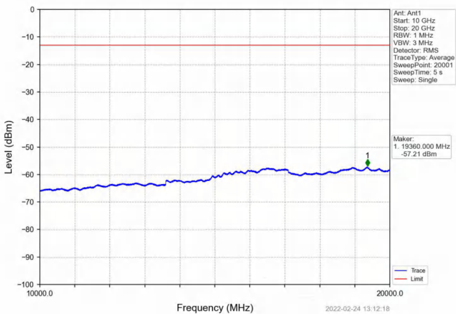
Band4_15MHz_16QAM_MCH_1732.5MHz_RB_1_0_NTNV
