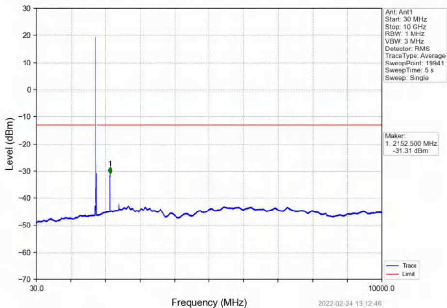
Band4_15MHz_QPSK_HCH_1747.5MHz_RB_1_0_NTNV
