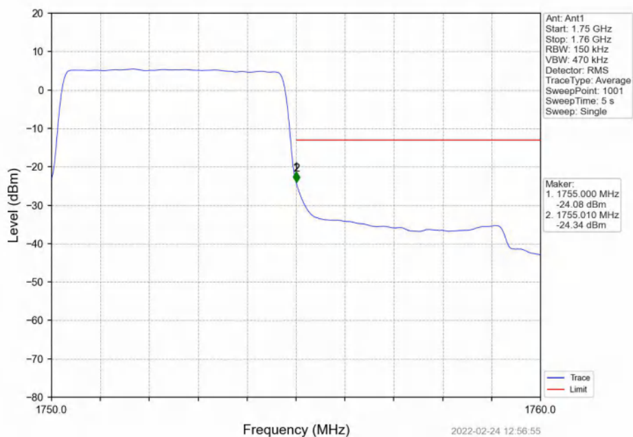
Band4_5MHz_QPSK_HCH_1752.5MHz_RB_25_0_NTNV
