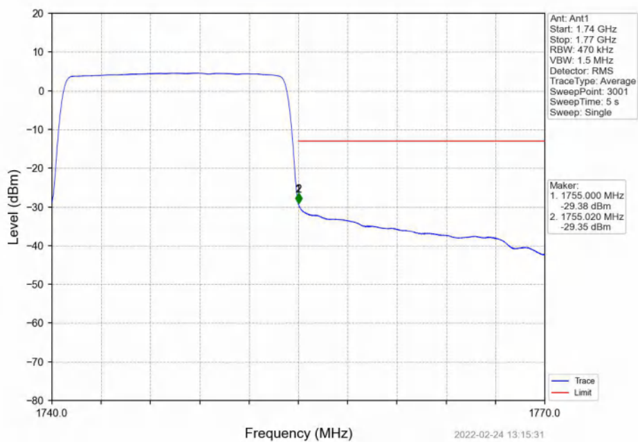
Band4_15MHz_16QAM_HCH_1747.5MHz_RB_75_0_NTNV
