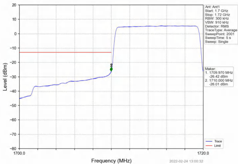
Band4_10MHz_QPSK_LCH_1715MHz_RB_50_0_NTNV
