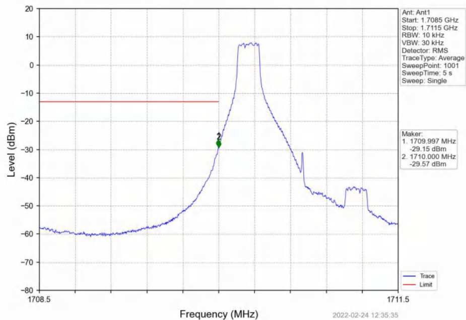
Band4_1.4MHz_16QAM_LCH_1710.7MHz_RB_1_0_NTNV
