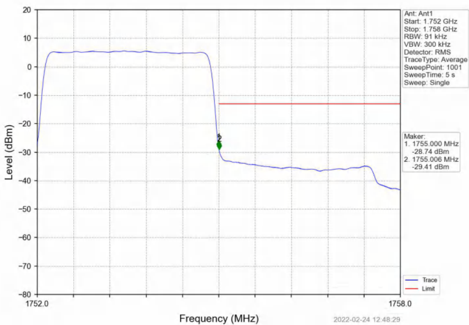
Band4_3MHz_QPSK_HCH_1753.5MHz_RB_15_0_NTNV
