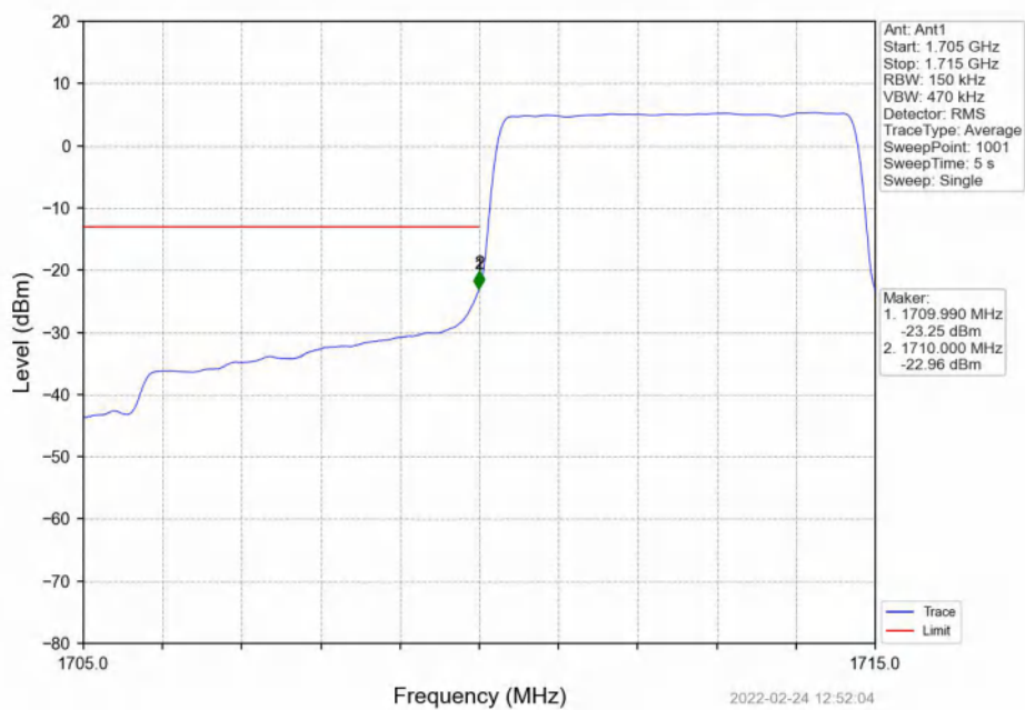
Band4_5MHz_QPSK_LCH_1712.5MHz_RB_25_0_NTNV
