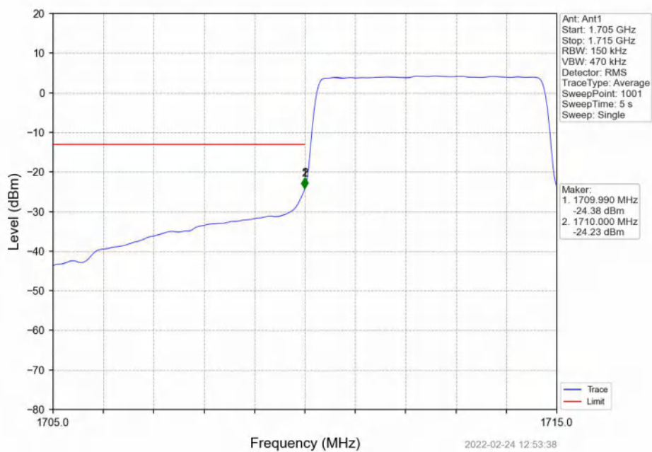
Band4_5MHz_16QAM_LCH_1712.5MHz_RB_25_0_NTNV
