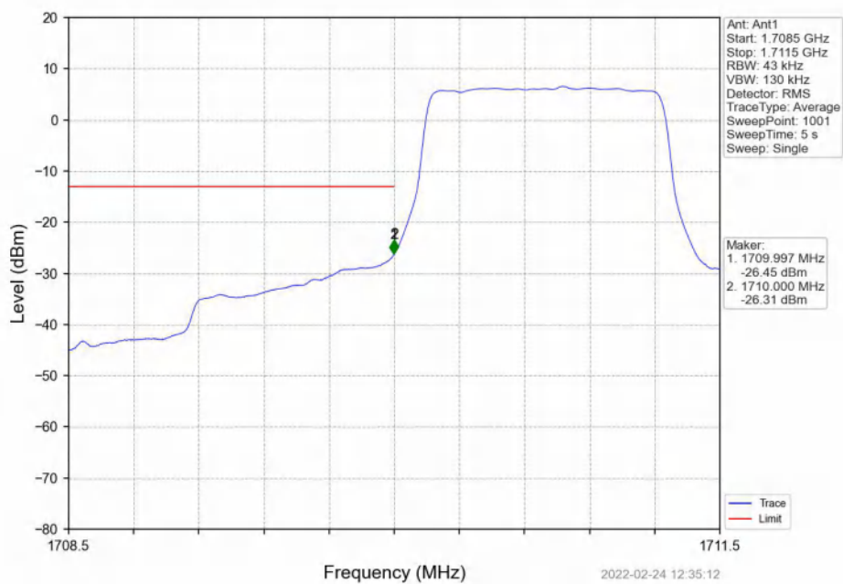
Band4_1.4MHz_QPSK_LCH_1710.7MHz_RB_6_0_NTNV
