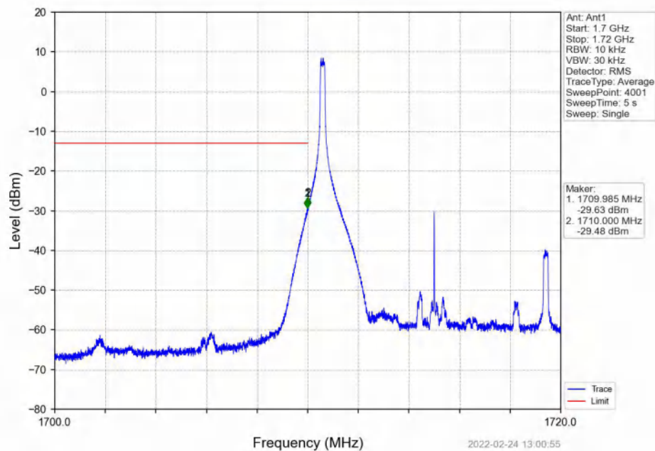
Band4_10MHz_16QAM_LCH_1715MHz_RB_1_0_NTNV
