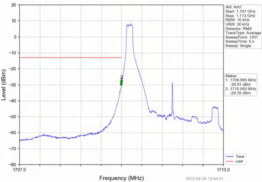
Band4_3MHz_16QAM_LCH_1711.5MHz_RB_1_0_NTNV
