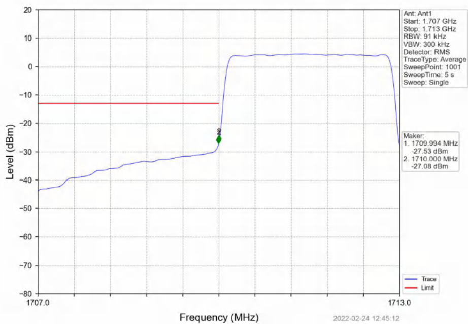
Band4_3MHz_16QAM_LCH_1711.5MHz_RB_15_0_NTNV
