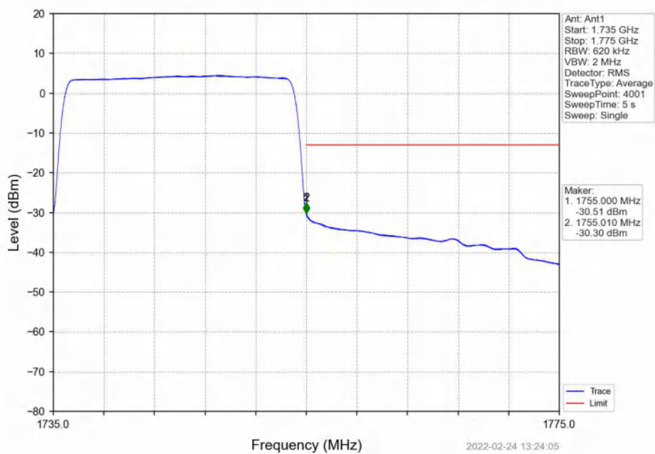
Band4_20MHz_16QAM_HCH_1745MHz_RB_100_0_NTNV
