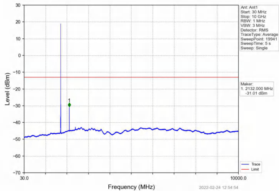
Band4_5MHz_16QAM_MCH_1732.5MHz_RB_1_0_NTNV
