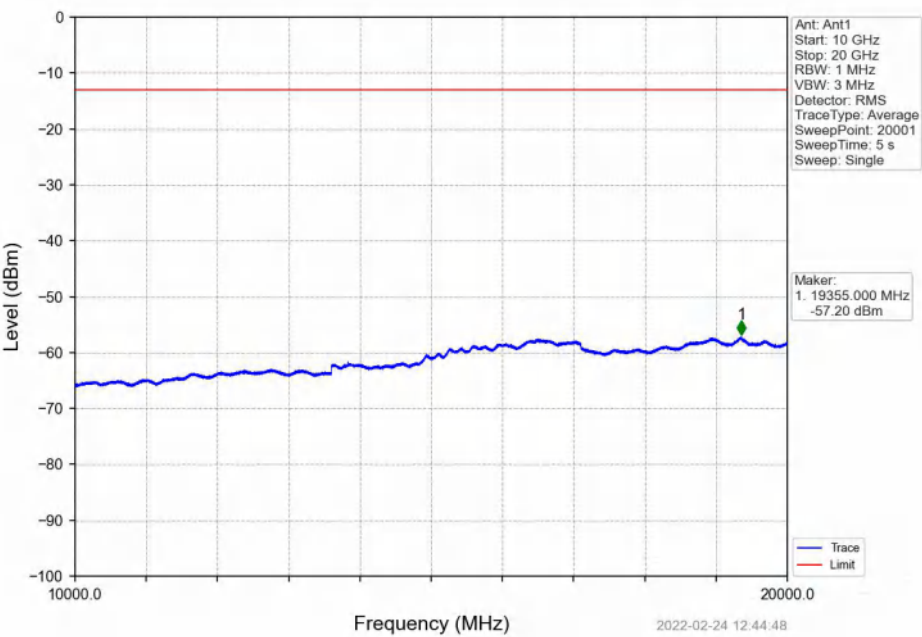
Band4_3MHz_16QAM_LCH_1711.5MHz_RB_15_0_NTNV
