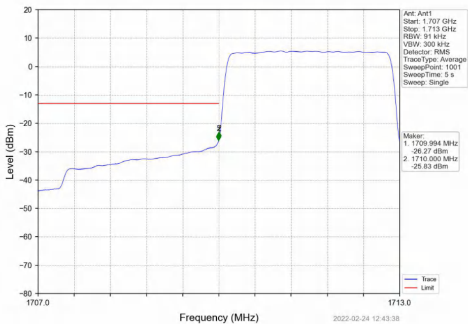
Band4_3MHz_QPSK_LCH_1711.5MHz_RB_15_0_NTNV
