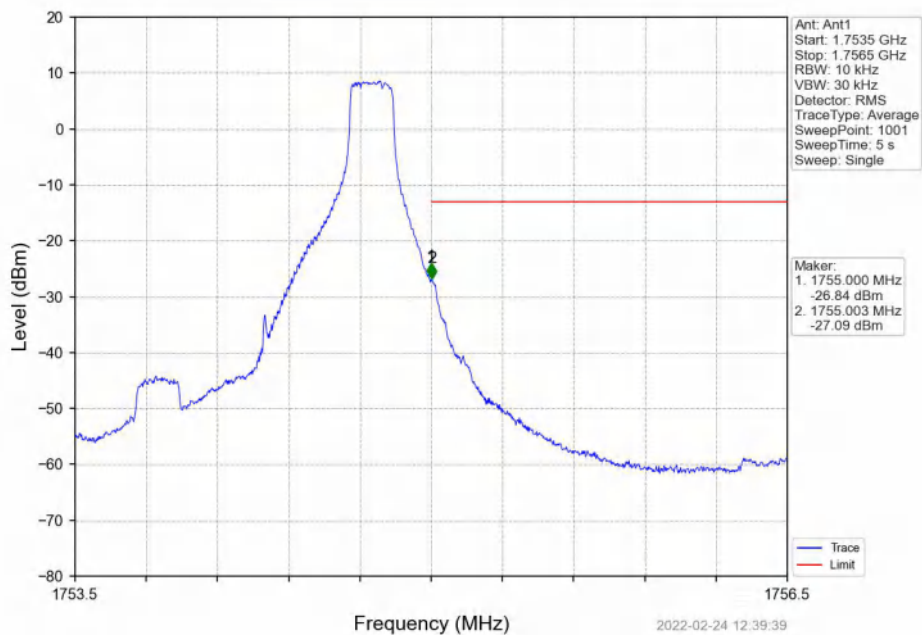
Band4_1.4MHz_QPSK_HCH_1754.3MHz_RB_6_0_NTNV
