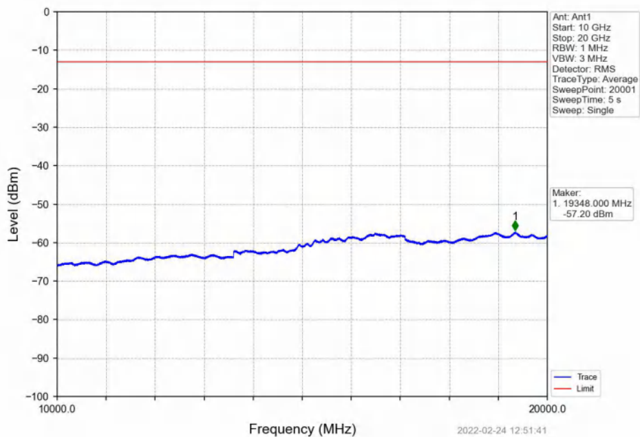
Band4_5MHz_QPSK_LCH_1712.5MHz_RB_25_0_NTNV
