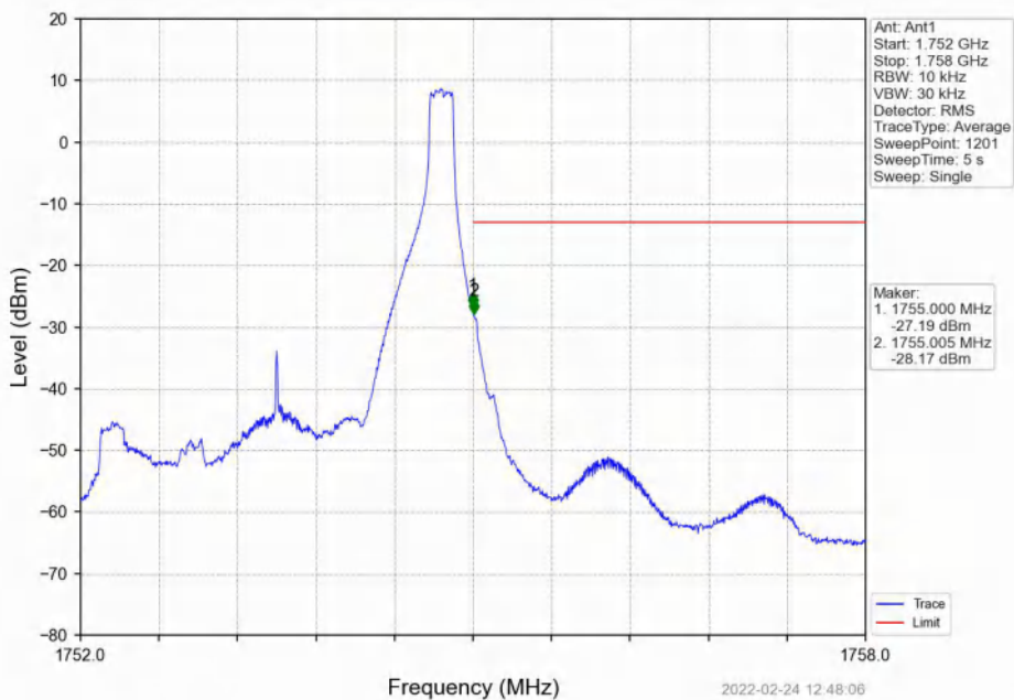
Band4_3MHz_QPSK_HCH_1753.5MHz_RB_15_0_NTNV
