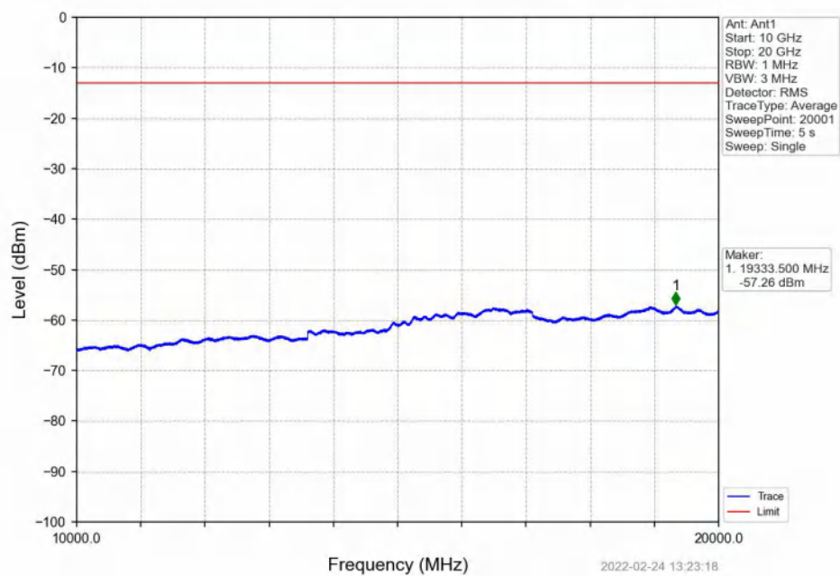
Band4_20MHz_16QAM_HCH_1745MHz_RB_1_0_NTNV
