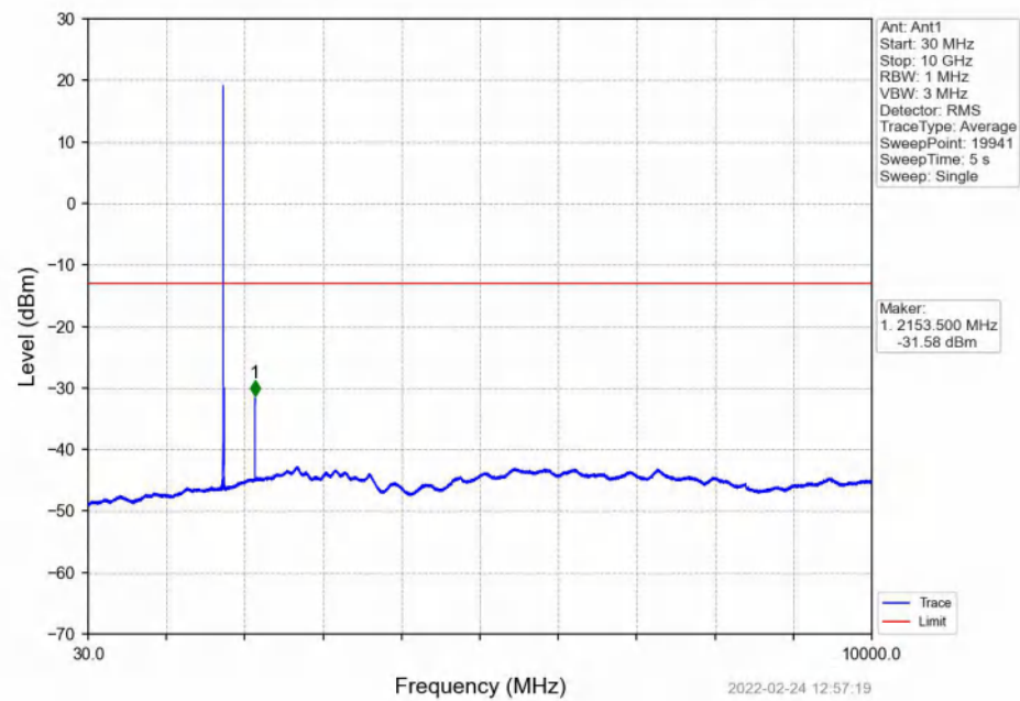
Band4_5MHz_16QAM_HCH_1752.5MHz_RB_1_0_NTNV
