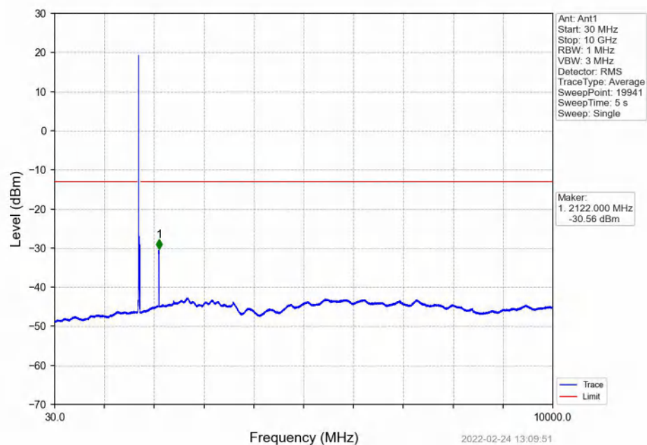
Band4_15MHz_16QAM_LCH_1717.5MHz_RB_1_0_NTNV
