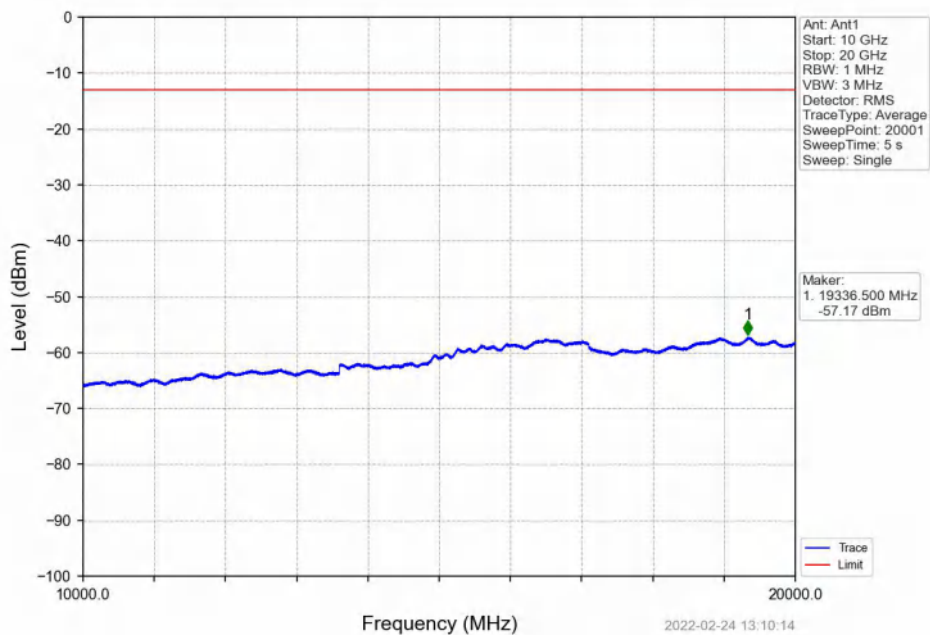
Band4_15MHz_16QAM_LCH_1717.5MHz_RB_75_0_NTNV
