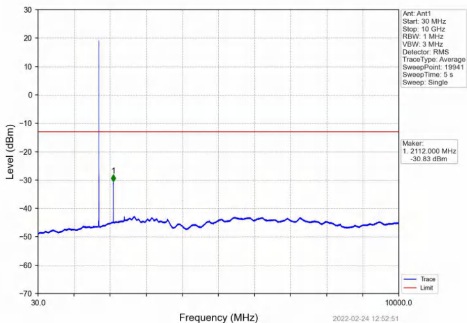
Band4_5MHz_16QAM_LCH_1712.5MHz_RB_1_0_NTNV
