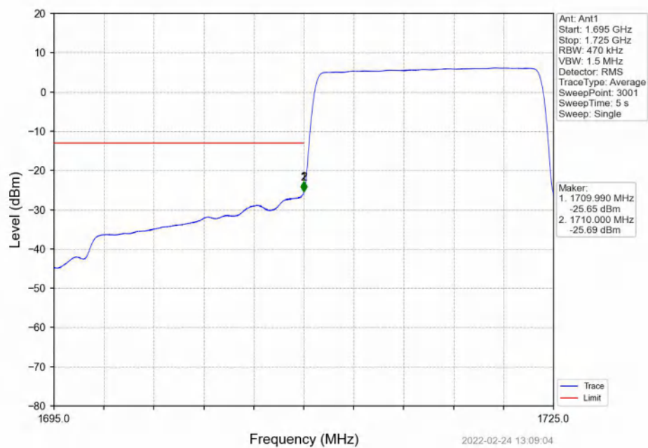
Band4_15MHz_QPSK_LCH_1717.5MHz_RB_75_0_NTNV
