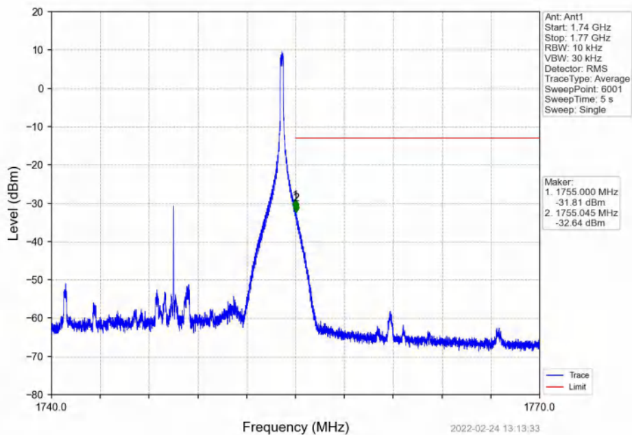
Band4_15MHz_QPSK_HCH_1747.5MHz_RB_75_0_NTNV
