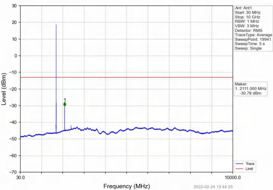
Band4_3MHz_16QAM_LCH_1711.5MHz_RB_1_0_NTNV
