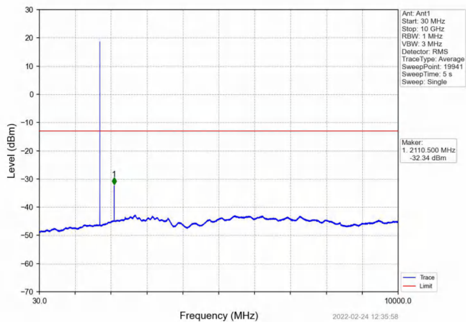
Band4_1.4MHz_16QAM_LCH_1710.7MHz_RB_1_0_NTNV
