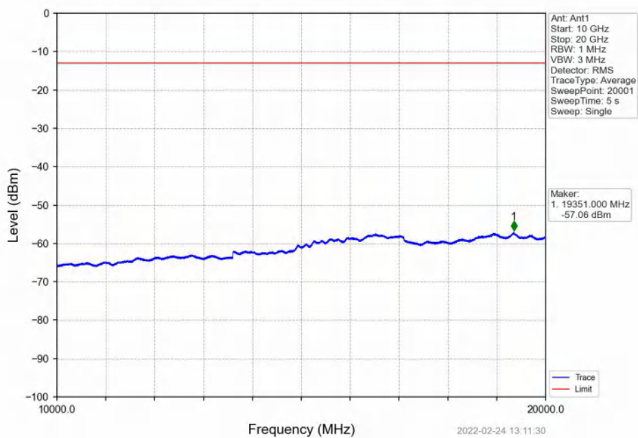
Band4_15MHz_QPSK_MCH_1732.5MHz_RB_1_0_NTNV
