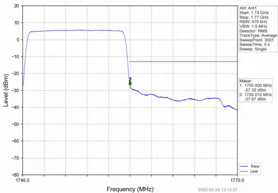
Band4_15MHz_QPSK_HCH_1747.5MHz_RB_75_0_NTNV
