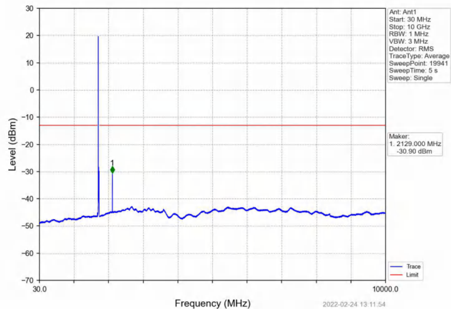
Band4_15MHz_16QAM_MCH_1732.5MHz_RB_1_0_NTNV
