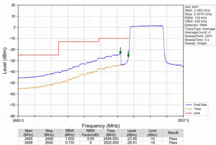
Band7_5MHz_16QAM_LCH_2502.5MHz_RB_25_0_NTNV
