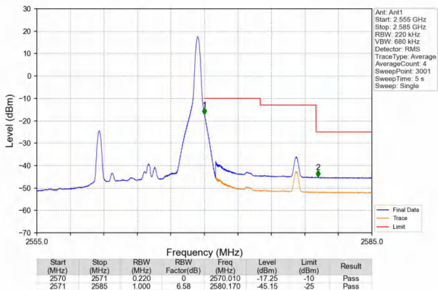
Band7_10MHz_16QAM_HCH_2565MHz_RB_1_49_NTNV
