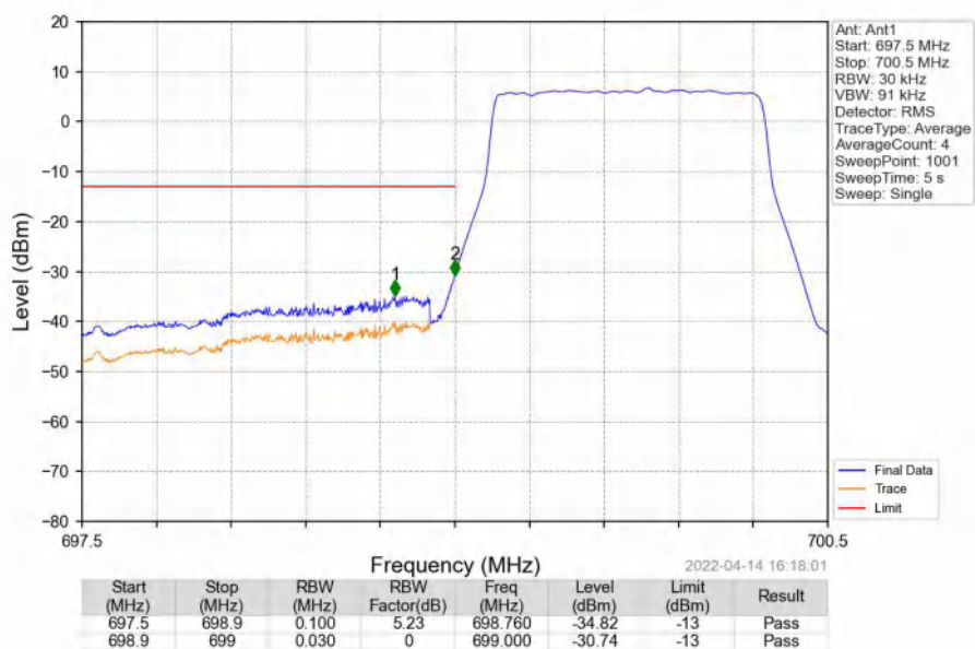
Band12_1.4MHz_QPSK_LCH_699.7MHz_RB_6_0_NTNV
