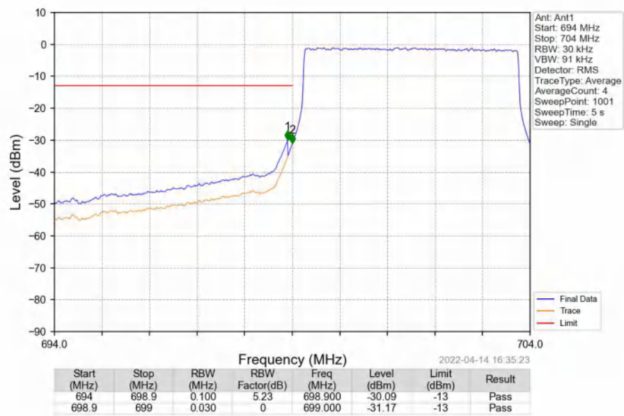
Band12_5MHz_16QAM_LCH_701.5MHz_RB_25_0_NTNV
