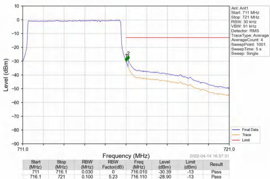
Band12_5MHz_QPSK_HCH_713.5MHz_RB_25_0_NTNV
