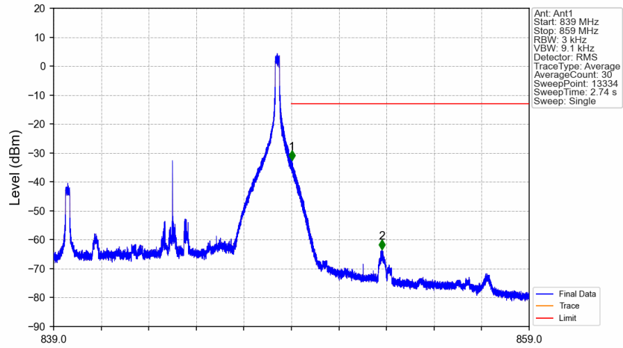
Band5 10MHz 16QAM HCH 844MHz RB 1 49 NTNV
