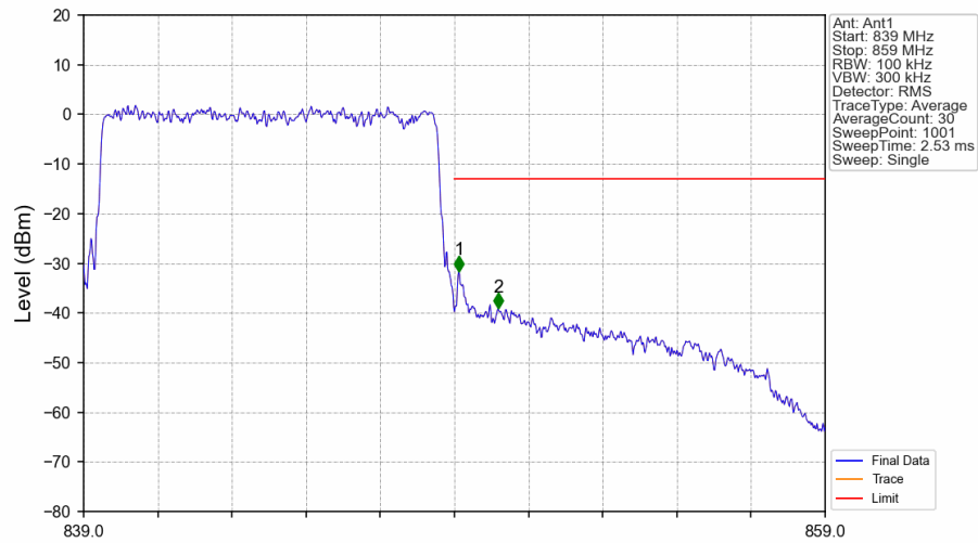
Band5 10MHz 16QAM HCH 844MHz RB 50 0 NTNV
