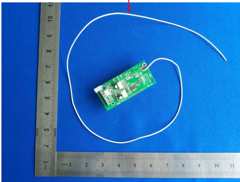
FM antenna
