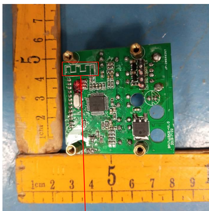
RF Antenna
