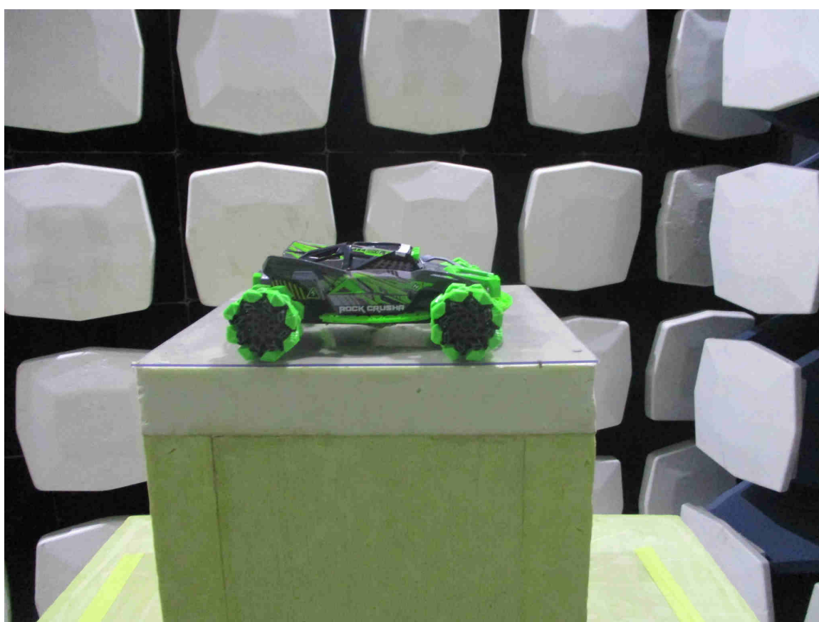
Above 1GHz (The EUT placed at the center of the turntable)
