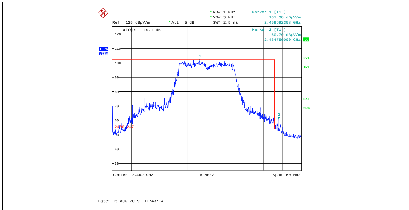
Plot 5.4.4.2.3.71. Band-Edge RF Radiated Emissions at 3 m, Horizontal Polarization, Peak 802.11n HT20, 400 ns, MCS 4, 16-QAM ¼ 43.3Mbps, Power Setting 18, Channel 11, 2462 MHz
