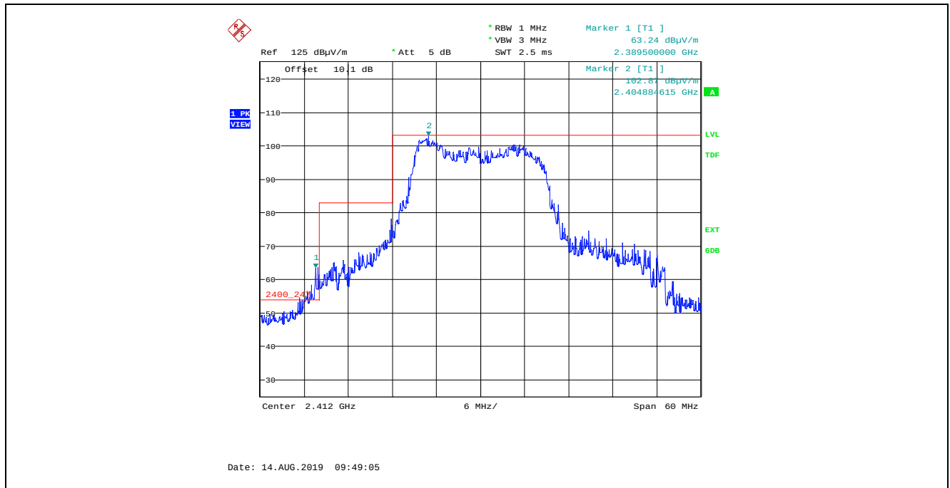
Plot 5.4.4.2.3.3. Band-Edge RF Radiated Emissions at 3 m, Horizontal Polarization, Peak 802.11n HT20, 400 ns, MCS 0, BPSK ½ 7.2Mbps, Power Setting 20, Channel 1, 2412 MHz
