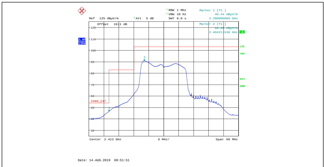
Plot 5.4.4.2.3.4. Band-Edge RF Radiated Emissions at 3 m, Horizontal Polarization, Average 802.11n HT20, 400 ns, MCS 0, BPSK ½ 7.2Mbps, Power Setting 20, Channel 1, 2412 MHz
