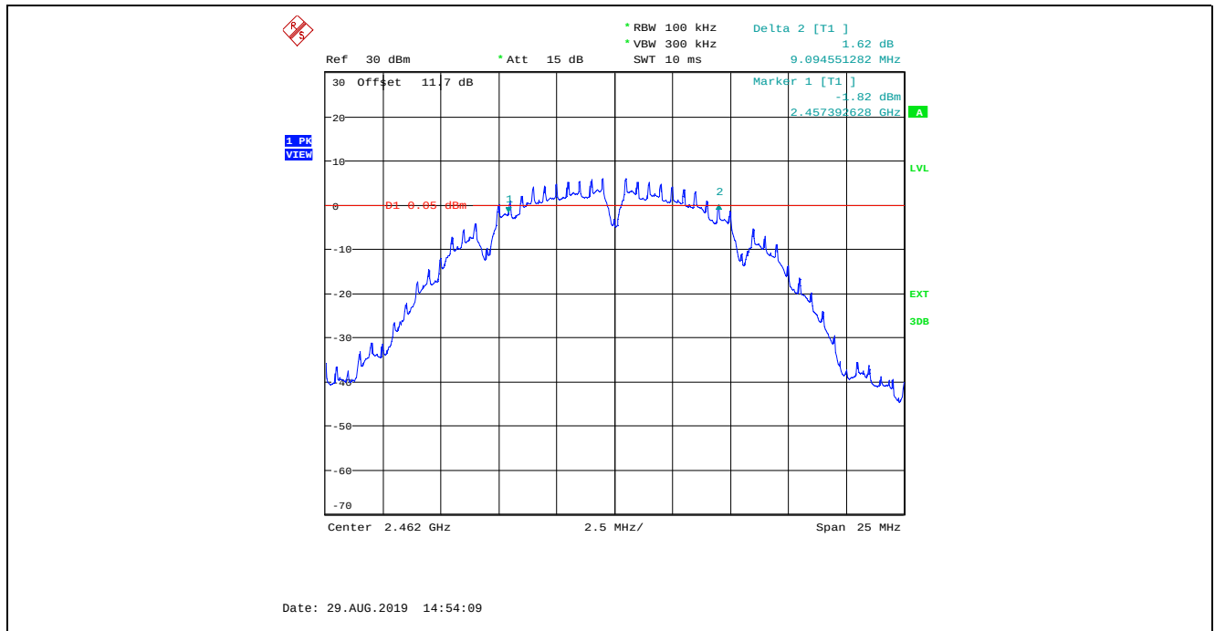
Plot 5.2.4.3. 6 dB Bandwidth 802.11b, DBPSK 1 Mbps, Power Setting 24, Channel 11, 2462 MHz
