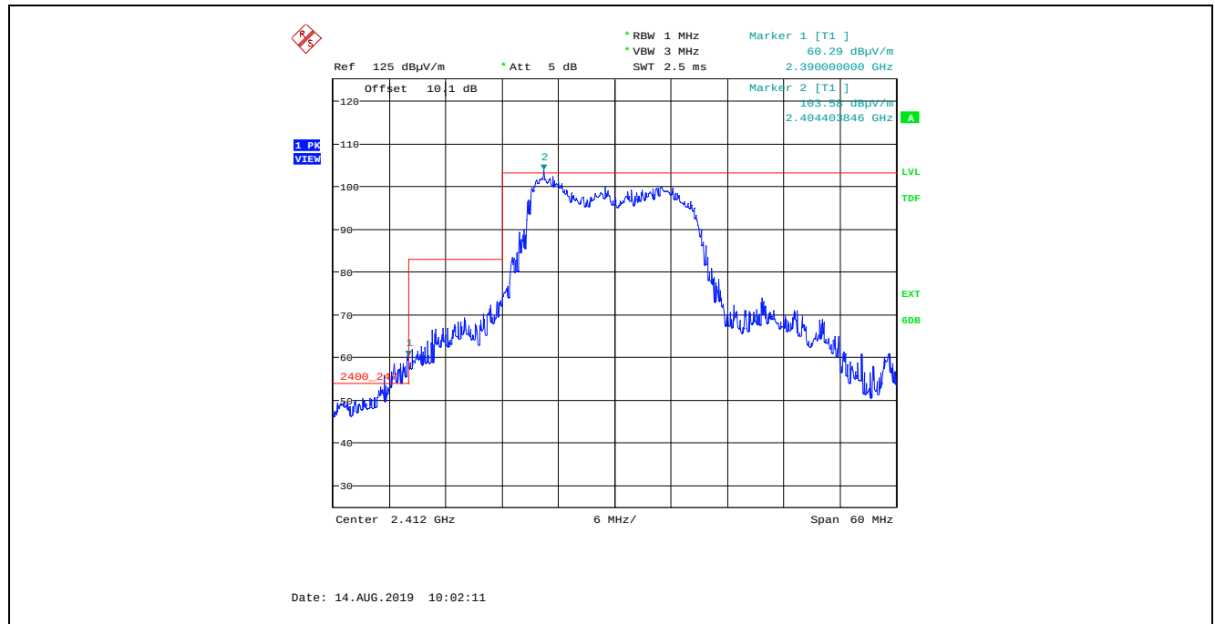
Plot 5.4.4.2.3.27. Band-Edge RF Radiated Emissions at 3 m, Horizontal Polarization, Peak 802.11n HT20, 400 ns, MCS 2, QPSK ¾ 21.7Mbps, Power Setting 20, Channel 1, 2412 MHz
