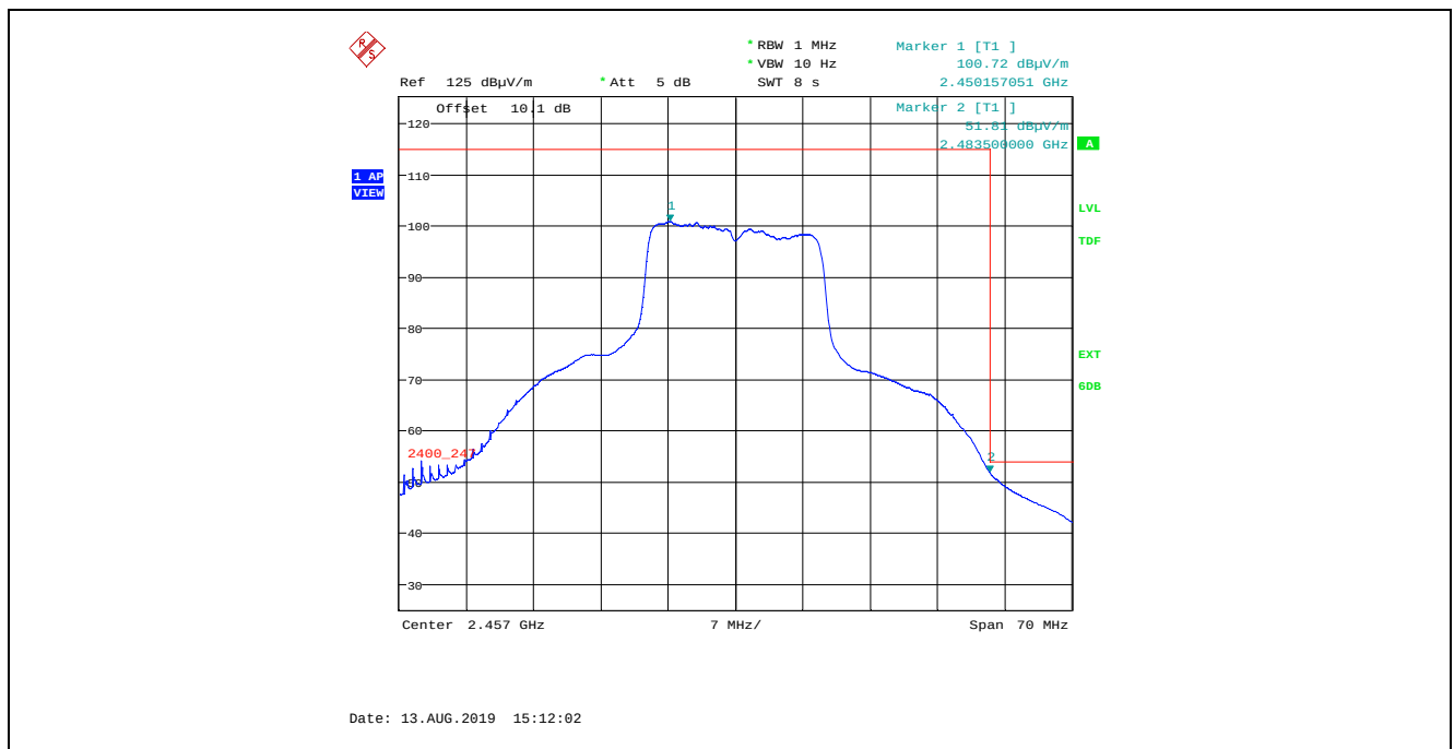
Plot 5.4.4.2.3.18. Band-Edge RF Radiated Emissions at 3 m, Vertical Polarization, Average 802.11n HT20, 400 ns, MCS 0, BPSK ½ 7.2Mbps, Power Setting 21, Channel 10, 2457 MHz
