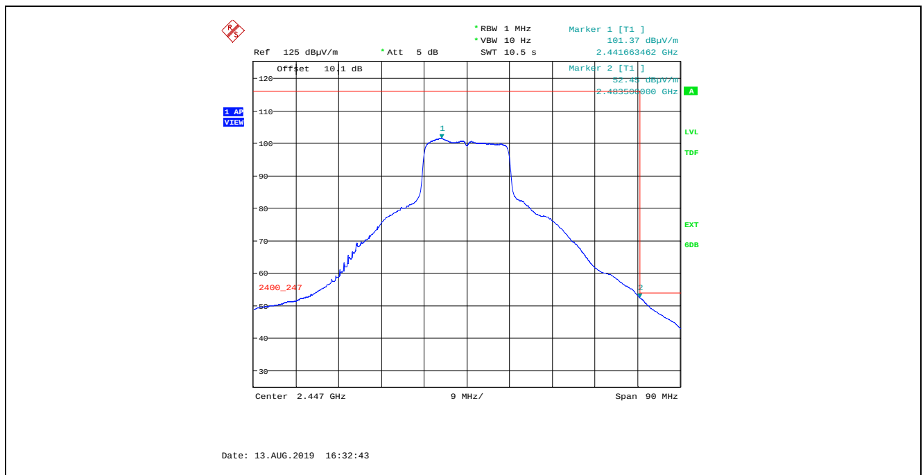
Plot 5.4.4.2.3.10. Band-Edge RF Radiated Emissions at 3 m, Vertical Polarization, Average 802.11n HT20, 400 ns, MCS 0, BPSK \frac{1}{2} 7.2Mbps, Power Setting 24, Channel 8, 2447 MHz
