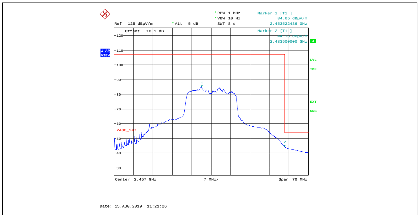
Plot 5.4.4.2.3.68. Band-Edge RF Radiated Emissions at 3 m, Horizontal Polarization, Average 802.11n HT20, 400 ns, MCS 4, 16-QAM \frac{3}{4} 43.3Mbps, Power Setting 21, Channel 10, 2457 MHz
