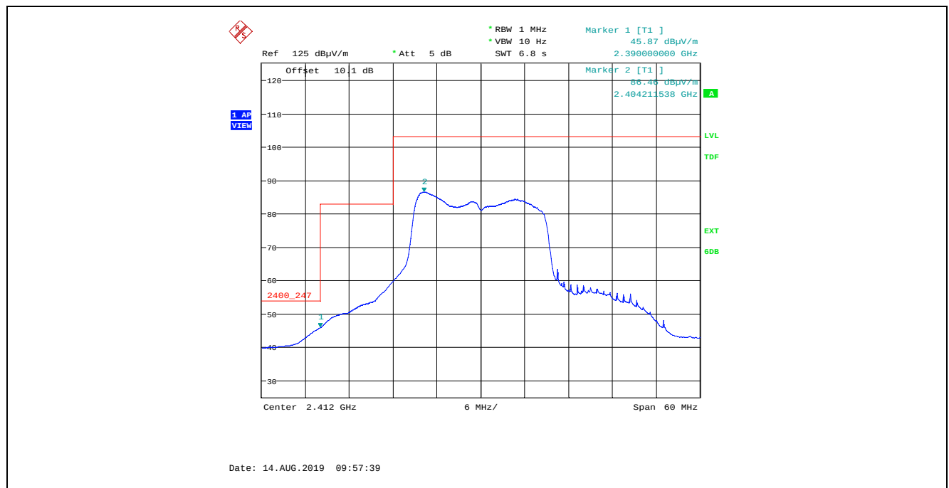
Plot 5.4.4.2.3.28. Band-Edge RF Radiated Emissions at 3 m, Horizontal Polarization, Average 802.11n HT20, 400 ns, MCS 2, QPSK ¾ 21.7Mbps, Power Setting 20, Channel 1, 2412 MHz
