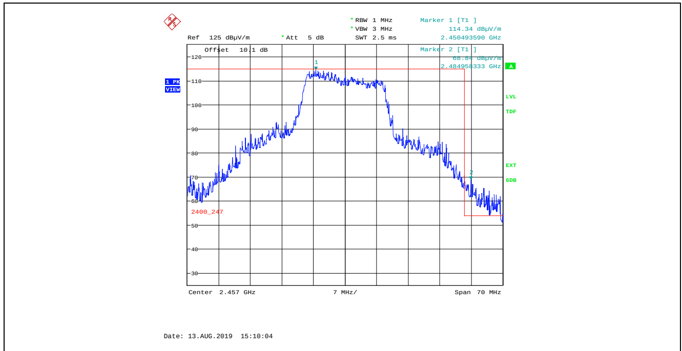
Plot 5.4.4.2.3.17. Band-Edge RF Radiated Emissions at 3 m, Vertical Polarization, Peak 802.11n HT20, 400 ns, MCS 0, BPSK ½ 7.2Mbps, Power Setting 21, Channel 10, 2457 MHz
