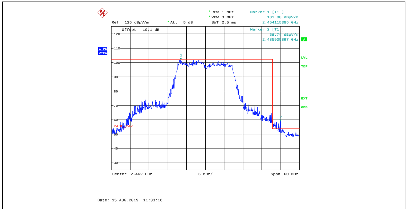
Plot 5.4.4.2.3.23. Band-Edge RF Radiated Emissions at 3 m, Horizontal Polarization, Peak 802.11n HT20, 400 ns, MCS 0, BPSK ½ 7.2Mbps, Power Setting 18, Channel 11, 2462 MHz
