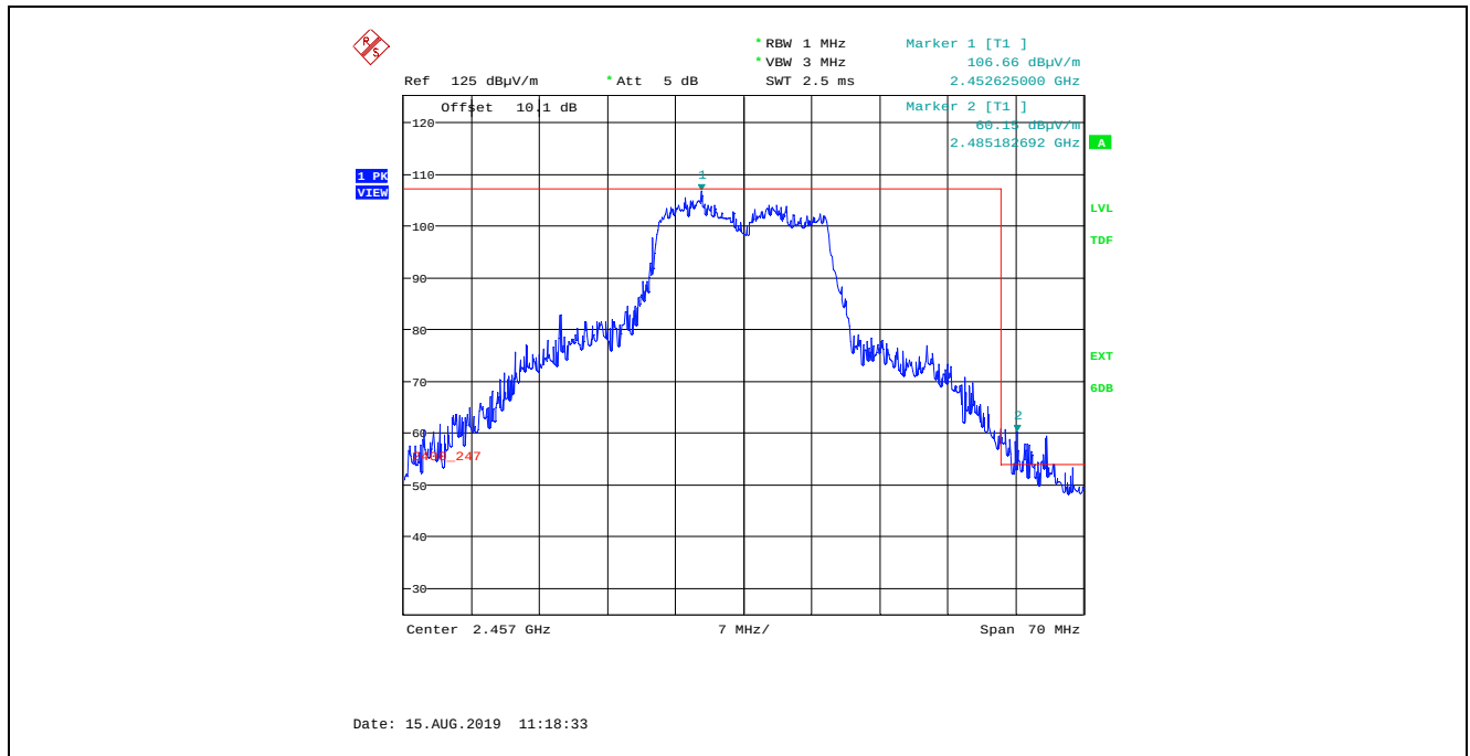
Plot 5.4.4.2.3.67. Band-Edge RF Radiated Emissions at 3 m, Horizontal Polarization, Peak 802.11n HT20, 400 ns, MCS 4, 16-QAM \frac{3}{4} 43.3Mbps, Power Setting 21, Channel 10, 2457 MHz
