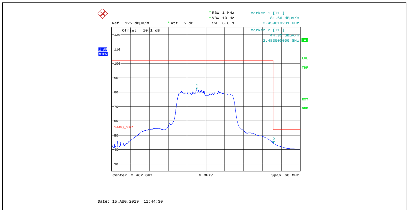
Plot 5.4.4.2.3.72. Band-Edge RF Radiated Emissions at 3 m, Horizontal Polarization, Average 802.11n HT20, 400 ns, MCS 4, 16-QAM ¼ 43.3Mbps, Power Setting 18, Channel 11, 2462 MHz
