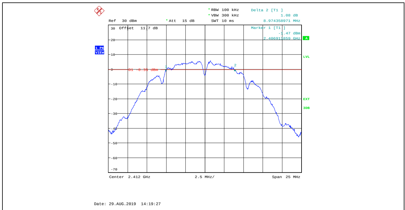
Plot 5.2.4.4. 6 dB Bandwidth 802.11b, DQPSK 2 Mbps, Power Setting 24, Channel 1, 2412 MHz,
