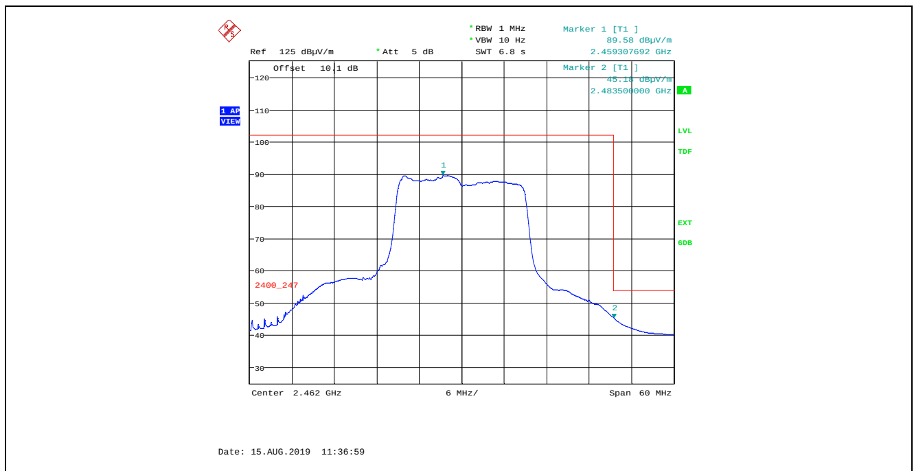
Plot 5.4.4.2.3.24. Band-Edge RF Radiated Emissions at 3 m, Horizontal Polarization, Average 802.11n HT20, 400 ns, MCS 0, BPSK ½ 7.2Mbps, Power Setting 18, Channel 11, 2462 MHz
