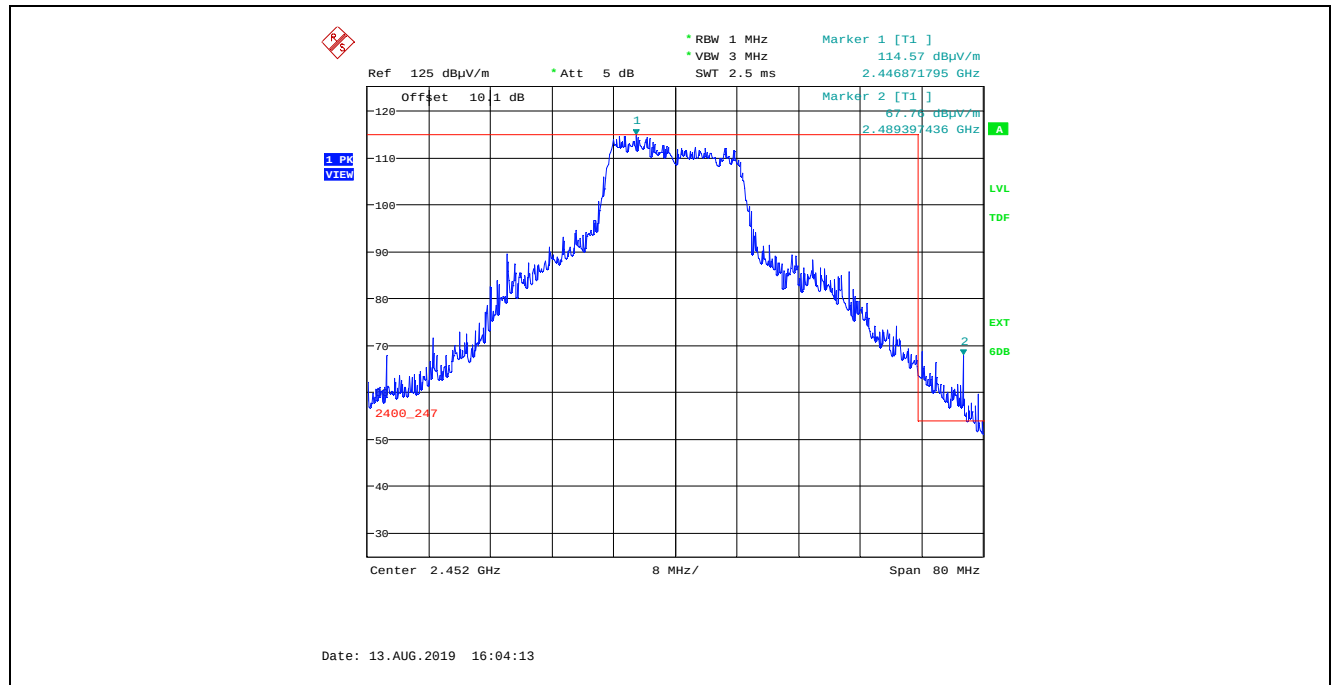
Plot 5.4.4.2.3.13. Band-Edge RF Radiated Emissions at 3 m, Vertical Polarization, Peak 802.11n HT20, 400 ns, MCS 0, BPSK ½ 7.2Mbps, Power Setting 21, Channel 9, 2452 MHz
