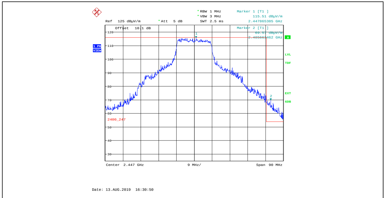
Plot 5.4.4.2.3.9. Band-Edge RF Radiated Emissions at 3 m, Vertical Polarization, Peak 802.11n HT20, 400 ns, MCS 0, BPSK \frac{1}{2} 7.2Mbps, Power Setting 24, Channel 8, 2447 MHz
