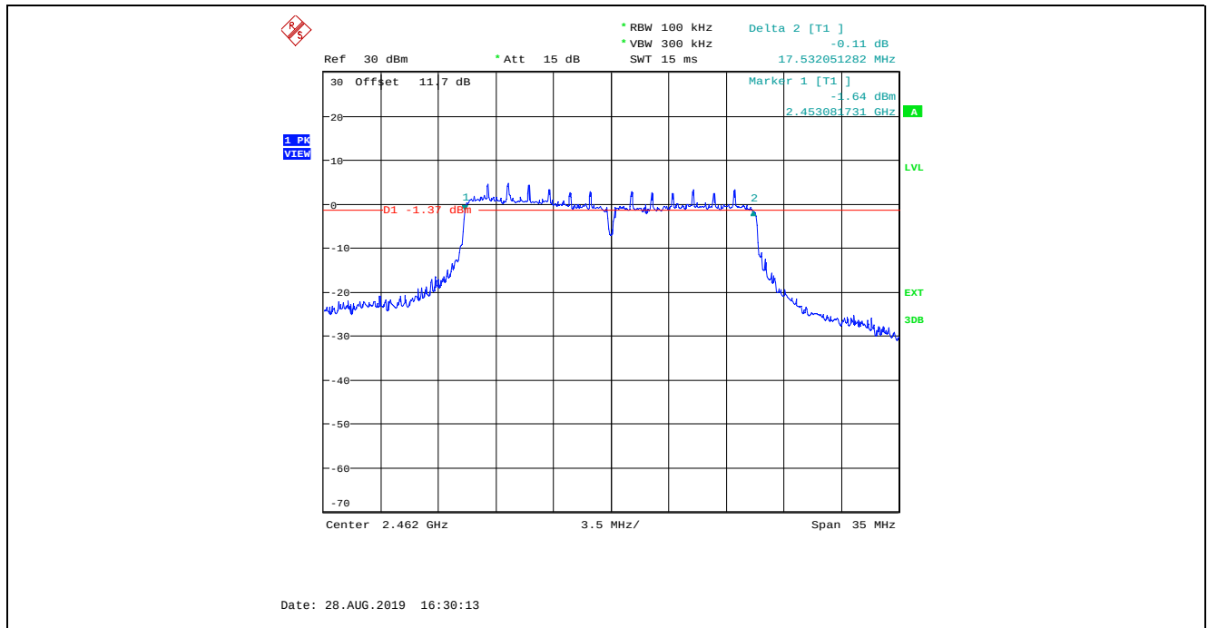
Plot 5.2.4.27. 6 dB Bandwidth 802.11n HT20, 400 ns, MCS 2, QPSK ¾ 21.7 Mbps, Power Setting 18, Channel 11, 2462 MHz
