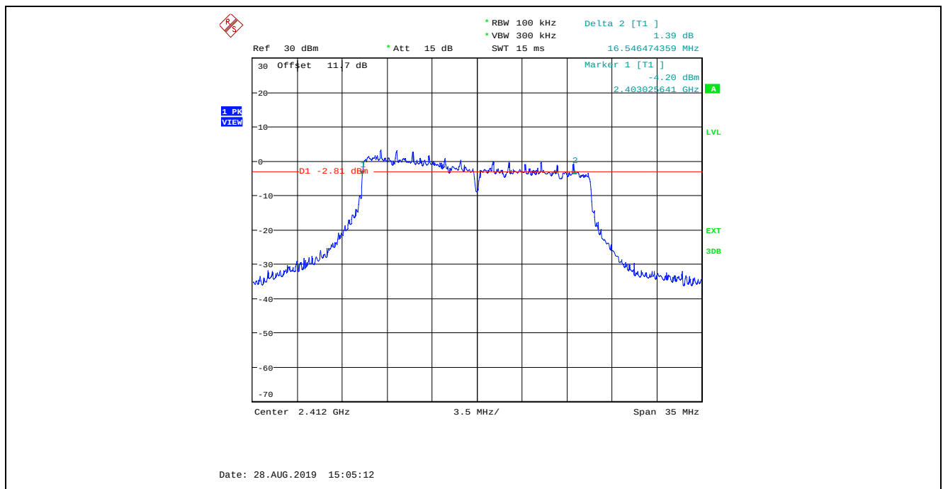
Plot 5.2.4.28. 6 dB Bandwidth 802.11n HT20, 400 ns, MCS 4, 16-QAM ¾ 43.3 Mbps, Power Setting 20, Channel 1, 2412 MHz
