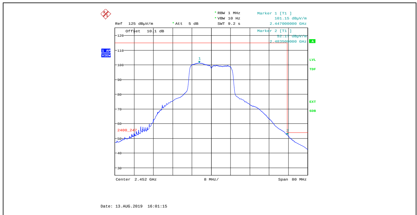
Plot 5.4.4.2.3.14. Band-Edge RF Radiated Emissions at 3 m, Vertical Polarization, Average 802.11n HT20, 400 ns, MCS 0, BPSK ½ 7.2Mbps, Power Setting 21, Channel 9, 2452 MHz
