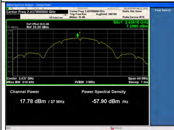
11b-PWR-Mid-1Mbps
