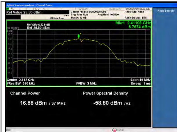
11b-PWR-Low-1Mbps
