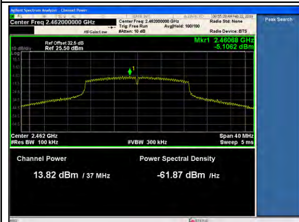
11n-20MHz-PSD-High-MCS0
