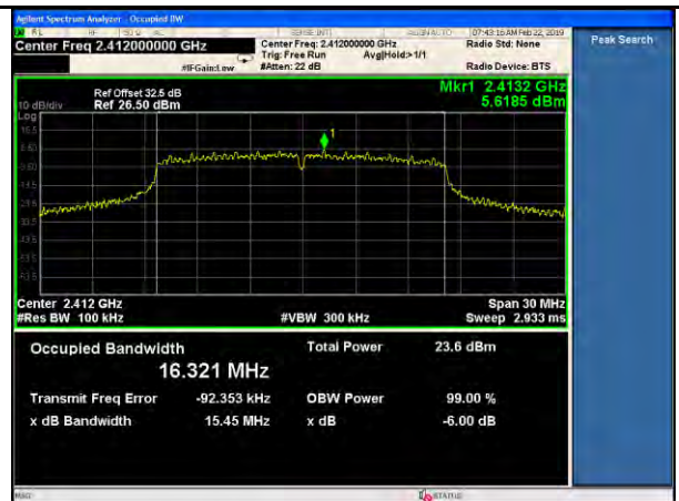
11g-6dB BW-Low-54Mbps
