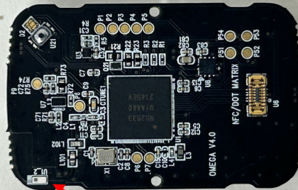
Chip Antenna
