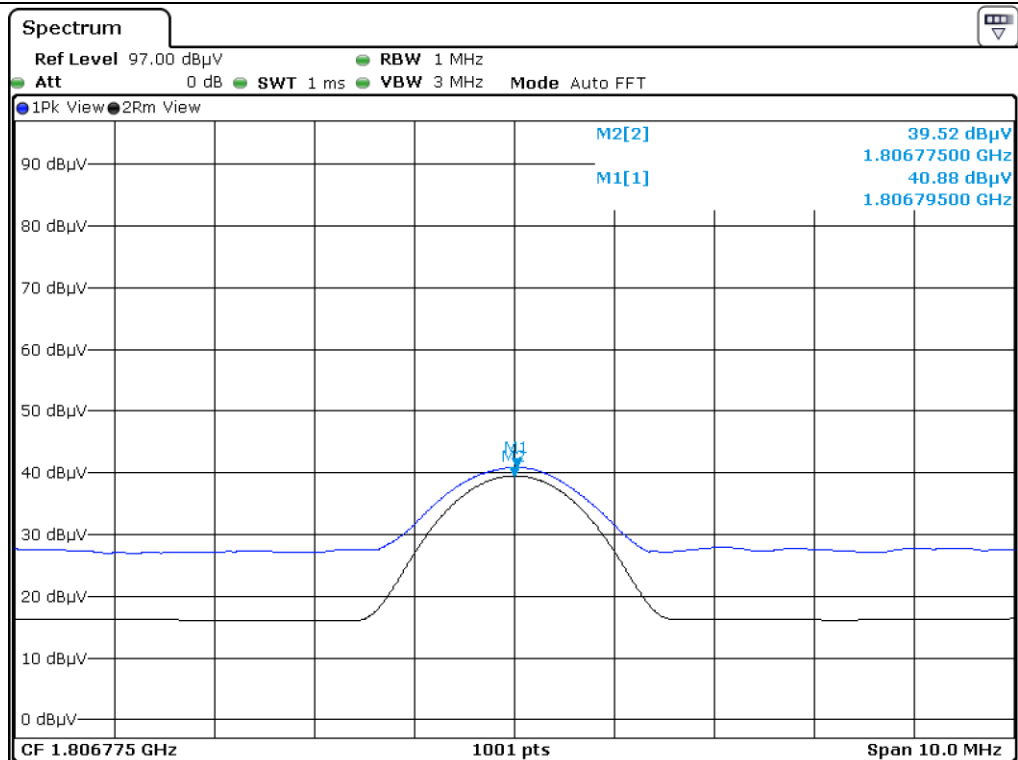
Middle Channel_H
