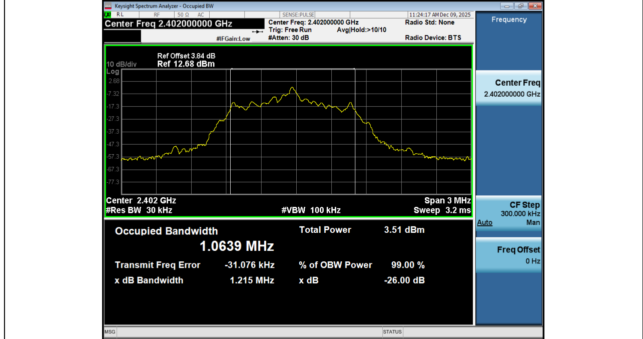
99% Occupied Bandwidth NVNT ANT1 1Mbps 2402
