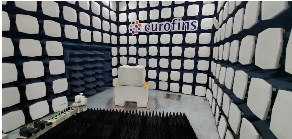
Picture 1 Radiated Emission Test Setup
