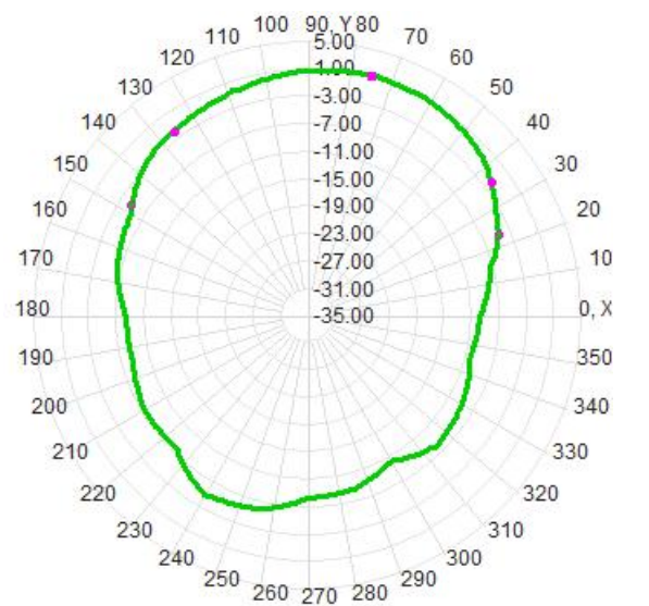
H面-THET=90
