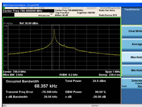
NB-IOT Band 13 QPSK 3.75kHz 1@0 CH-High
