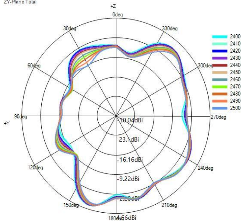
ZY-Plane Total
