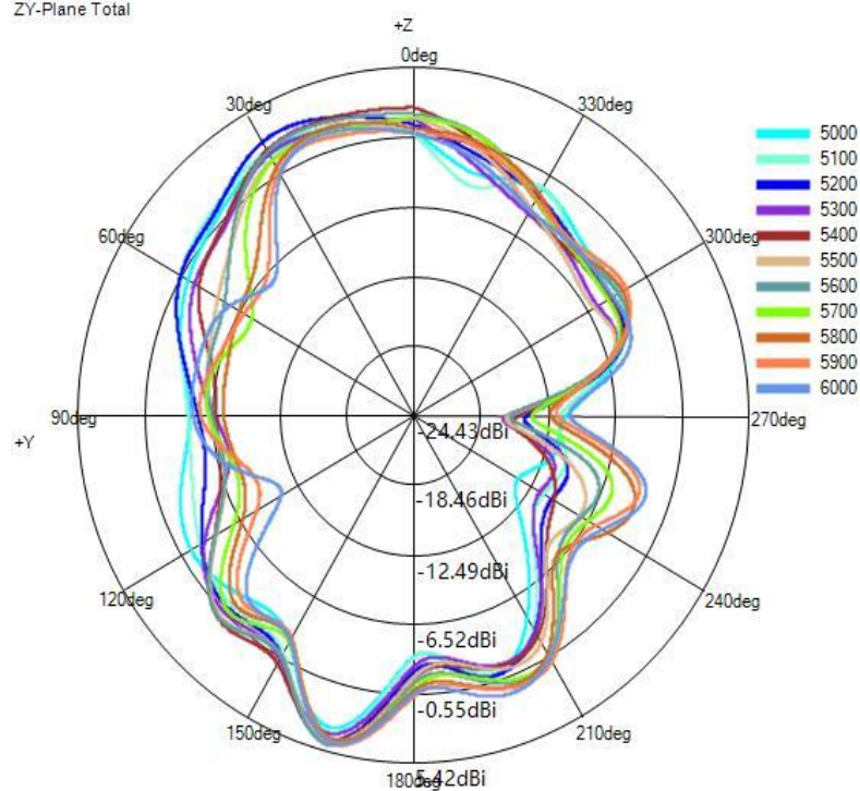
ZY-Plane Total
