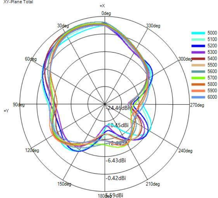
XY-Plane Total
