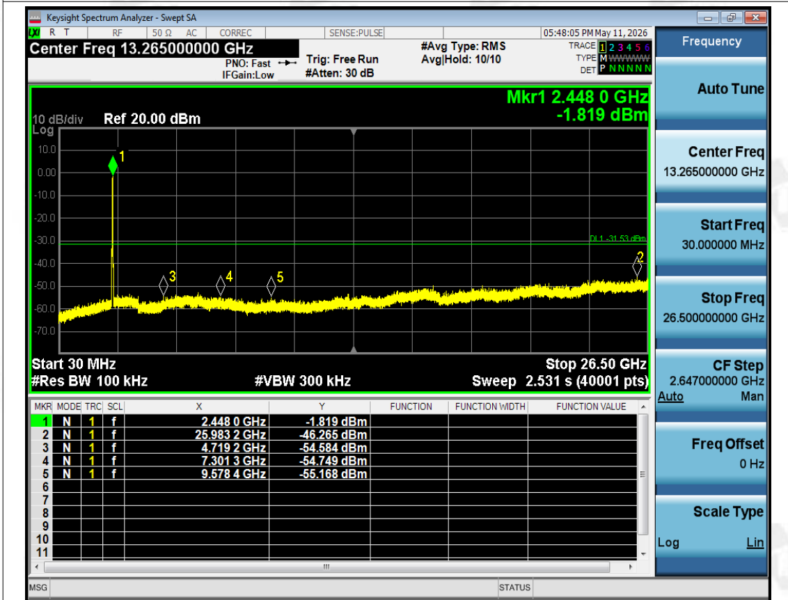
Tx. Spurious NVNT ax40 2437MHz Ant1 Emission
