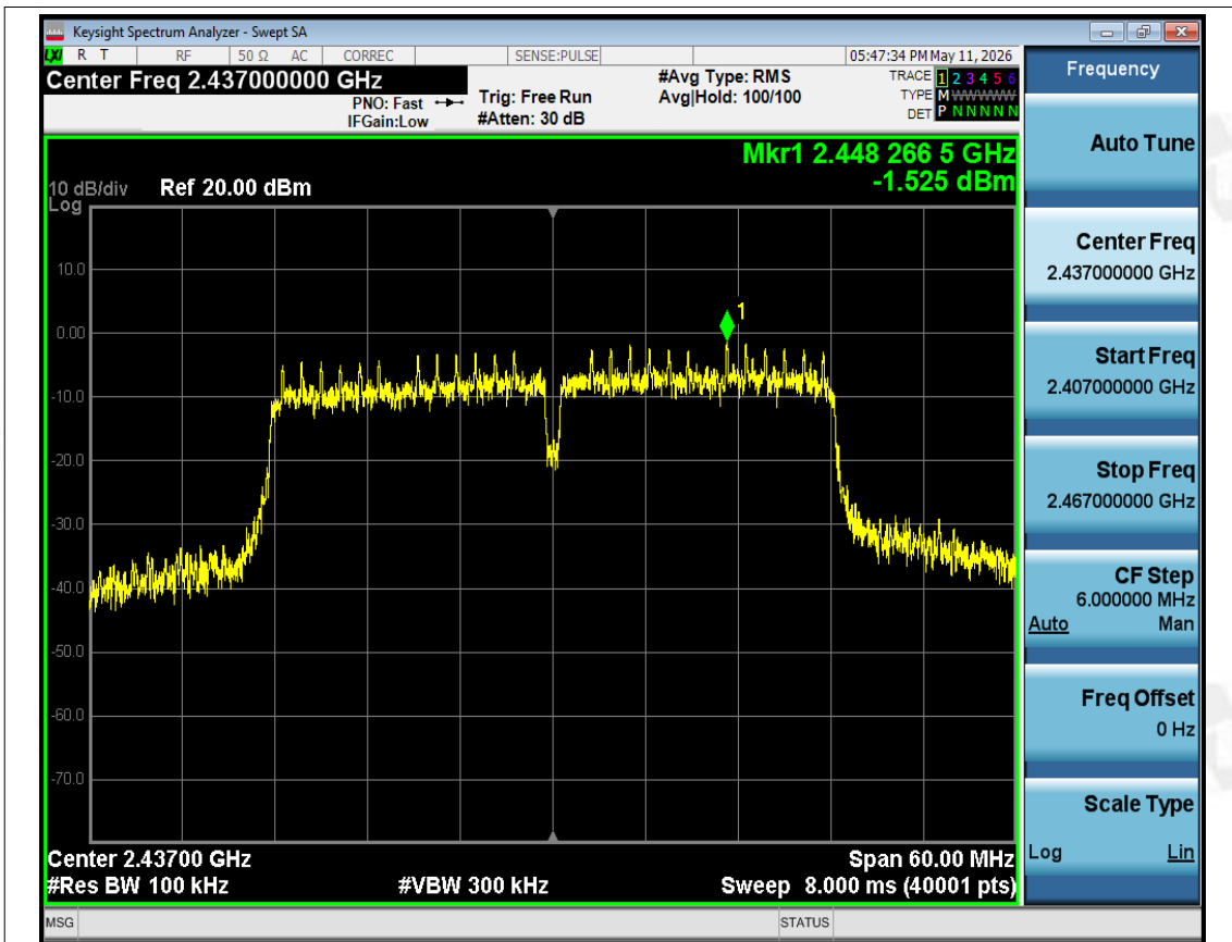
Tx. Spurious NVNT ax40 2437MHz Ant1 Ref
