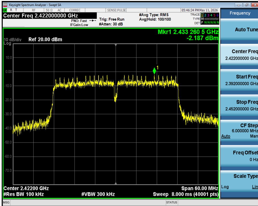
Tx. Spurious NVNT ax40 2422MHz Ant1 Ref
