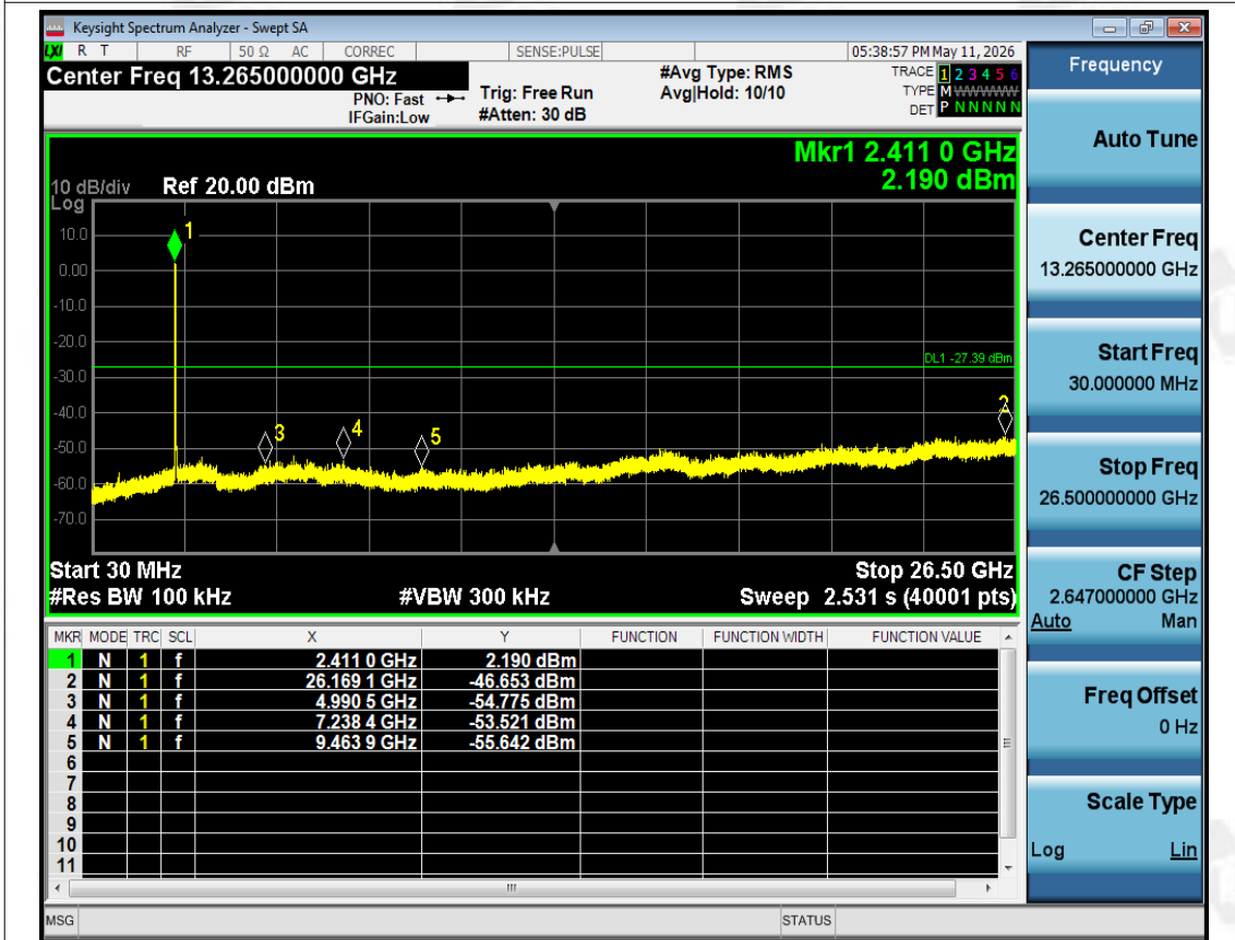
Tx. Spurious NVNT ax20 2412MHz Ant1 Emission
