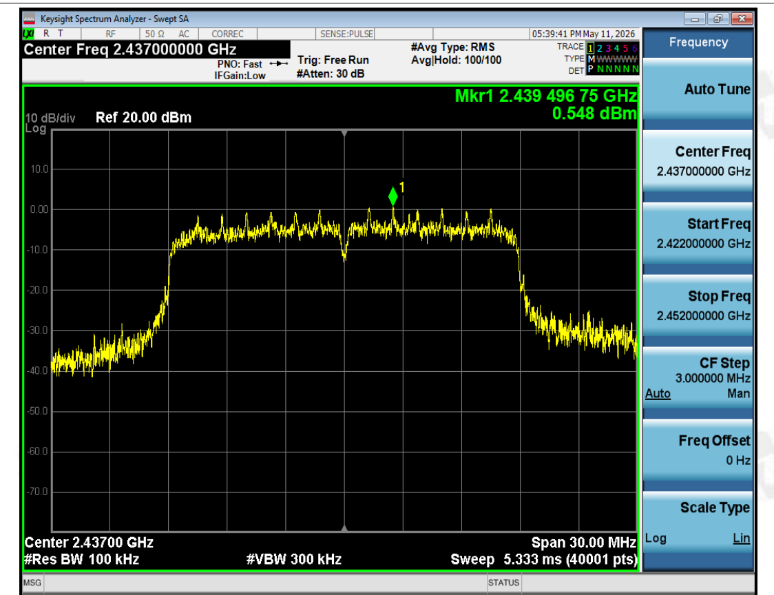
Tx. Spurious NVNT ax20 2437MHz Ant1 Ref
