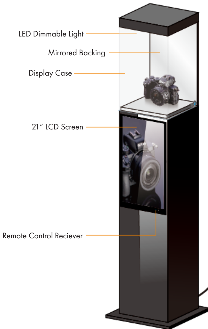
Side View
