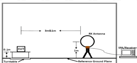
Figure 1. Below 30MHz
