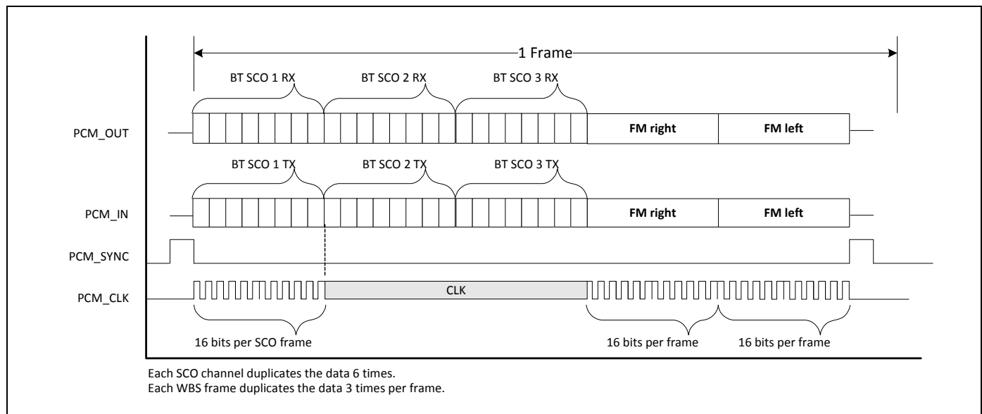
Figure 22. Functional Multiplex Data Diagram
