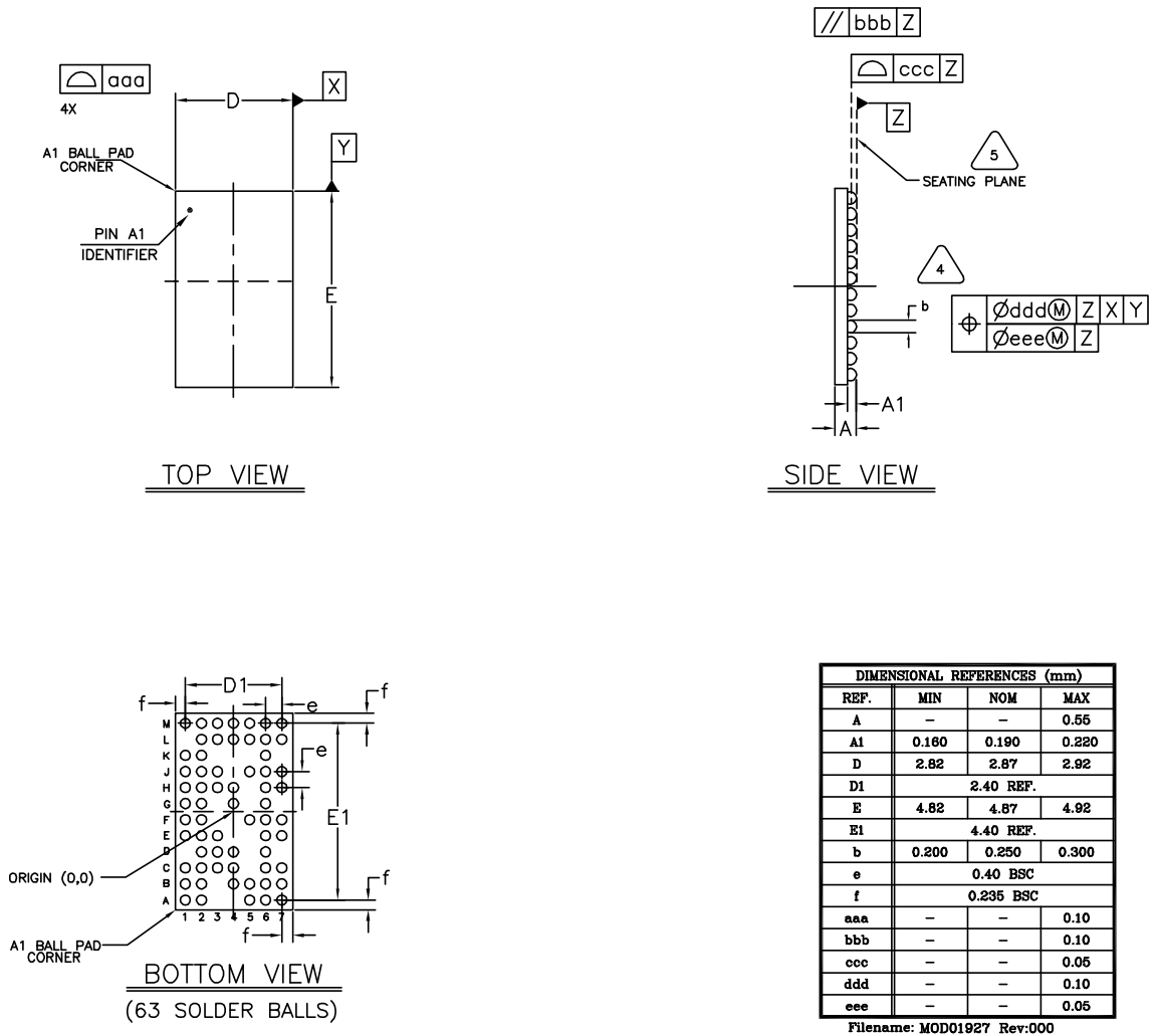
Figure 42. 63-Ball WLBGA Mechanical Information
