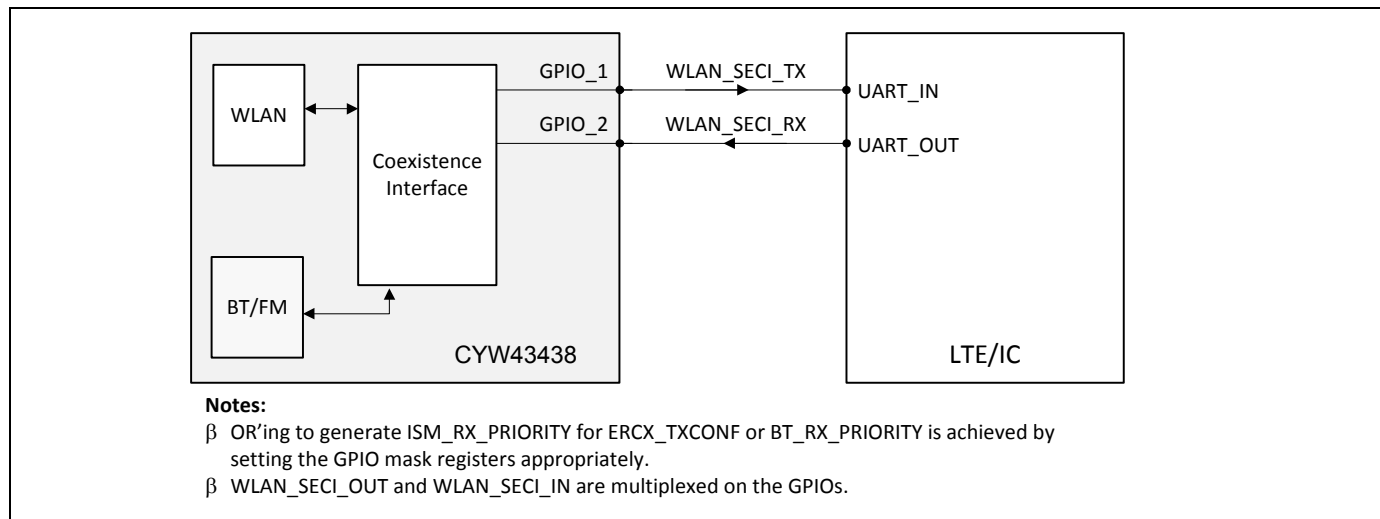
Figure 31. 2-Wire Coexistence Interface to an LTE IC
