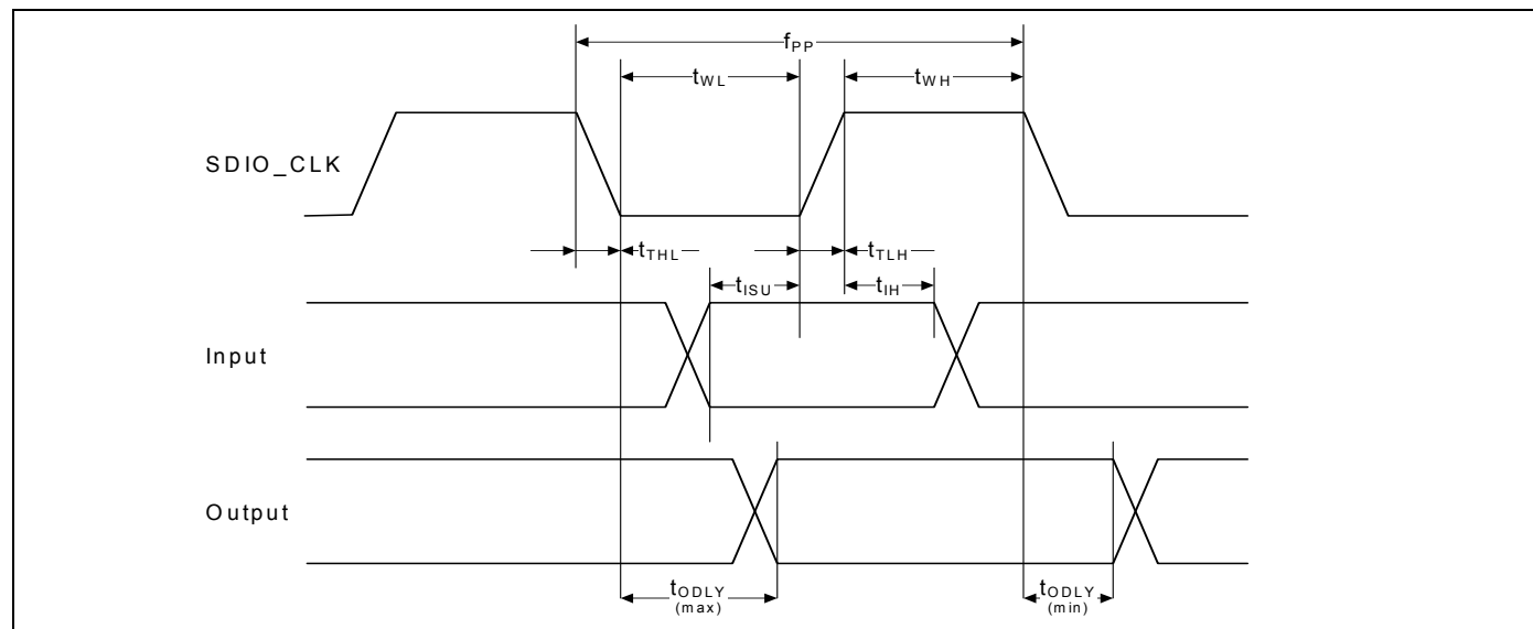
Figure 35. SDIO Bus Timing (Default Mode)
