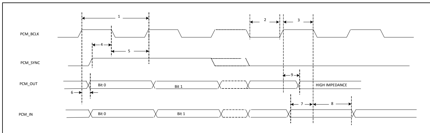
Figure 26. PCM Timing Diagram (Long Frame Sync, Slave Mode)
