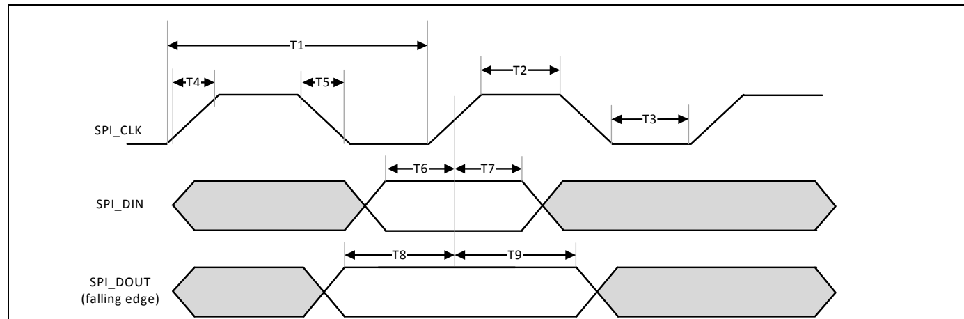
Figure 37. gSPI Timing
