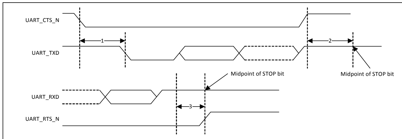
Figure 27. UART Timing
