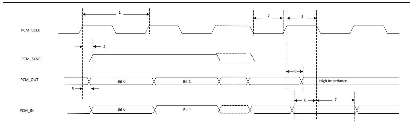
Figure 25. PCM Timing Diagram (Long Frame Sync, Master Mode)
