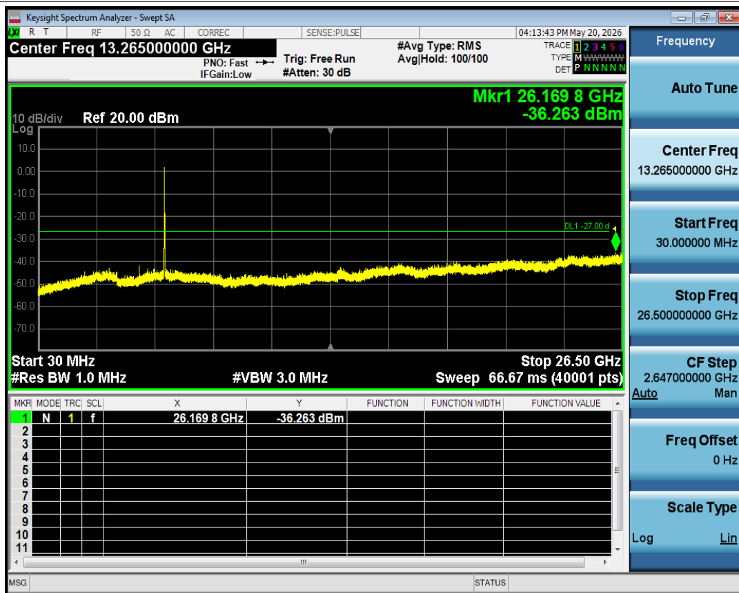
Tx. Spurious NVNT ax20 5745MHz Ant1 Emission
