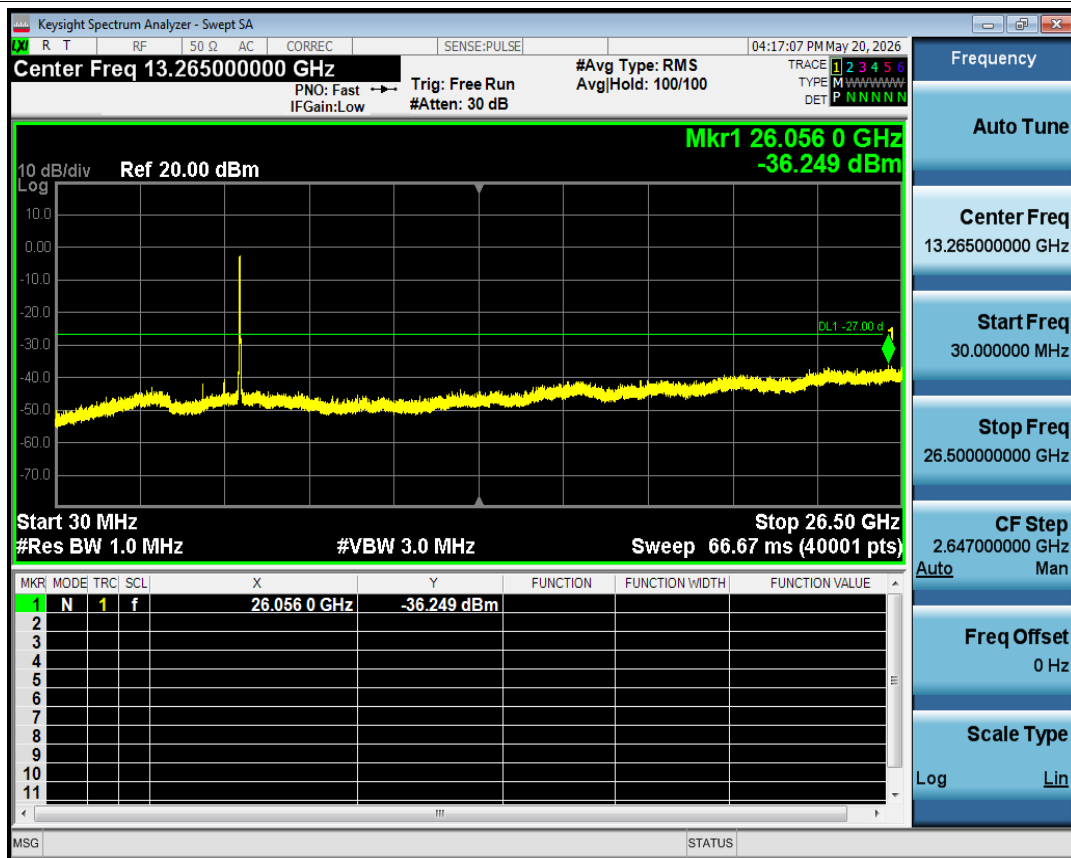
Tx. Spurious NVNT ac40 5795MHz Ant1 Emission
