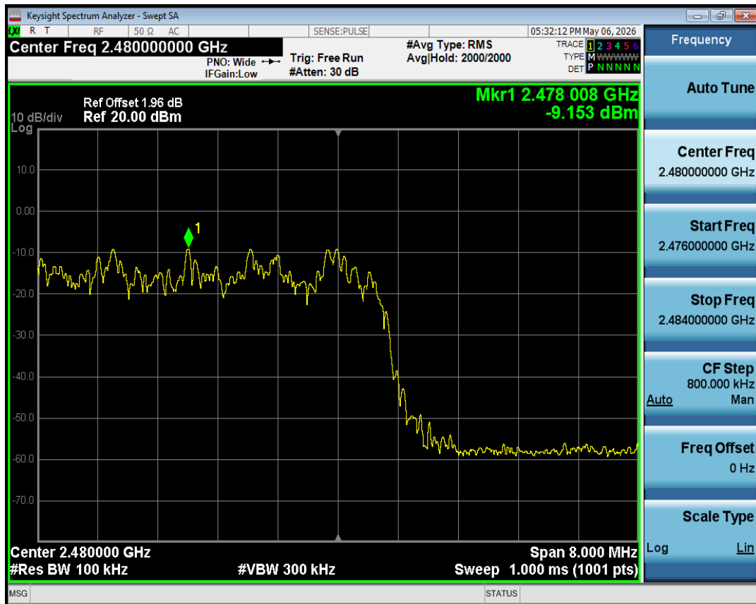
Band Edge(Hopping) NVNT 2-DH1 2480MHz Ant1 Hopping Ref
