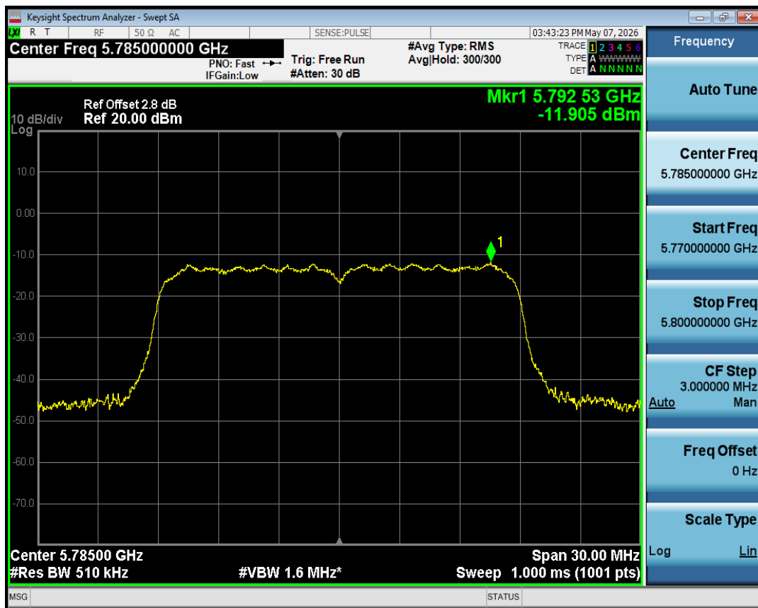
PSD NVNT n20 5785MHz Ant1
