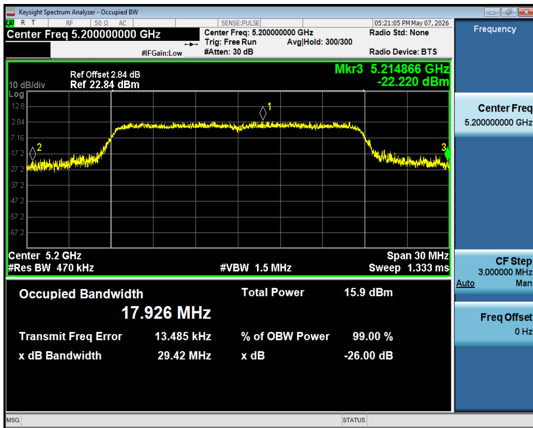
-26dB Bandwidth NVNT n20 5200MHz Ant1
