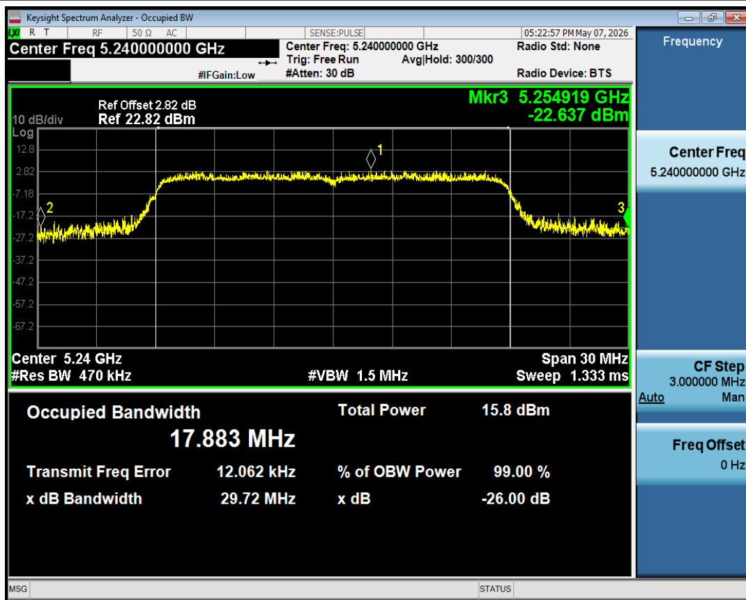
-26dB Bandwidth NVNT n20 5240MHz Ant1
