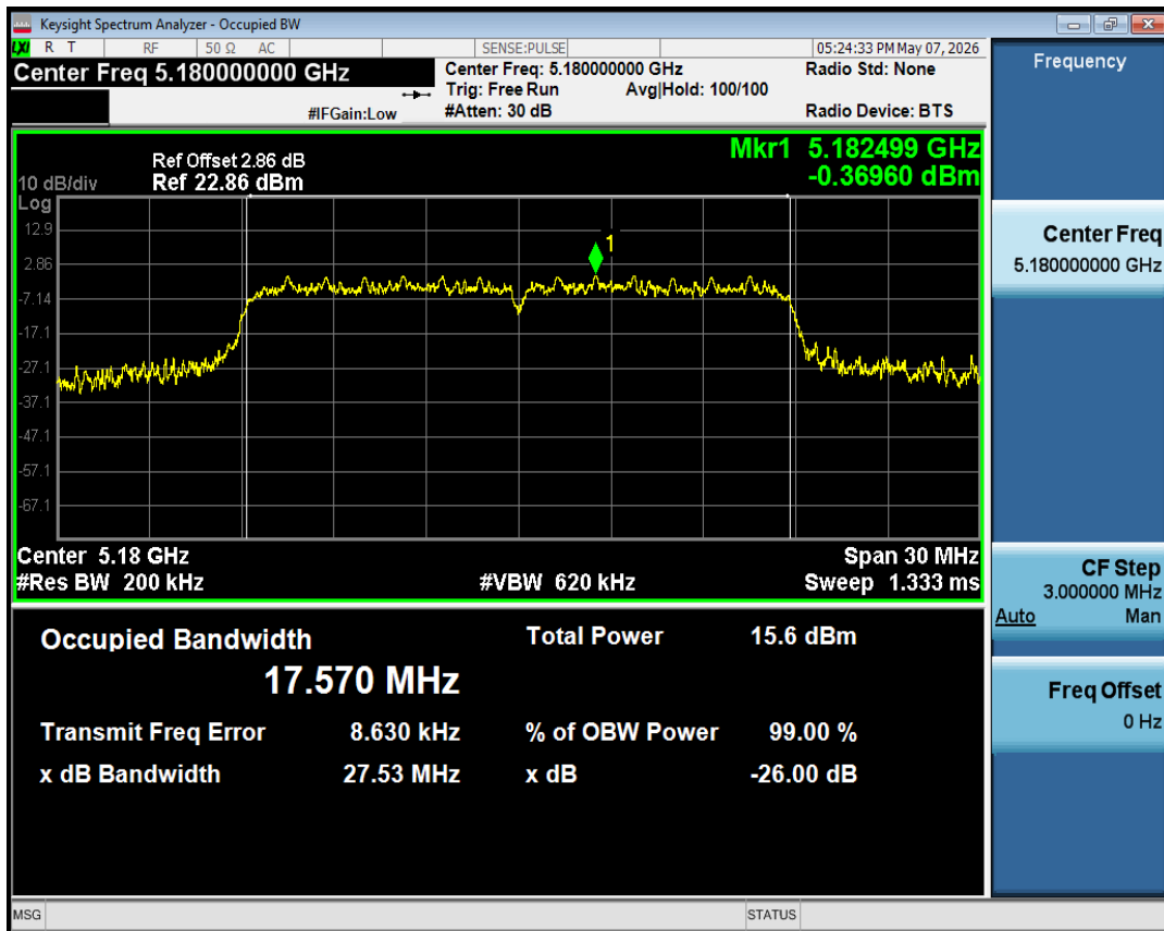
OBW NVNT ac20 5180MHz Ant1
