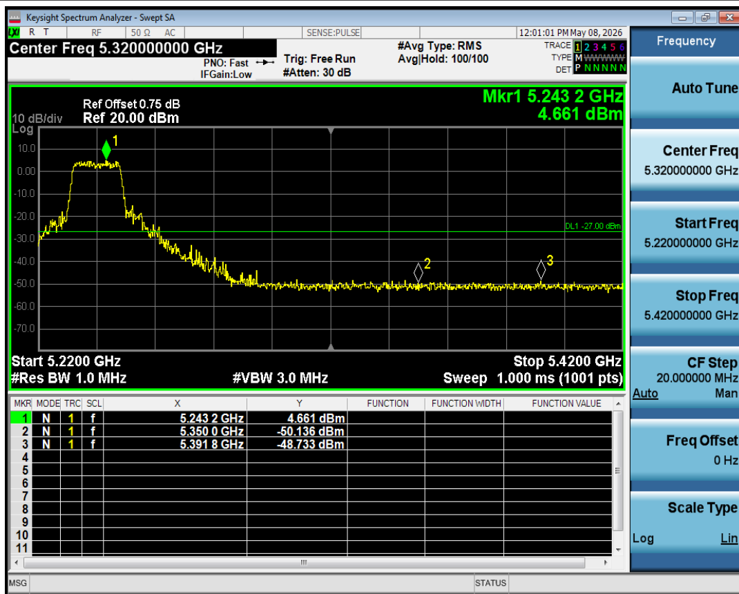
Band Edge NVNT a 5240MHz High Ant1
