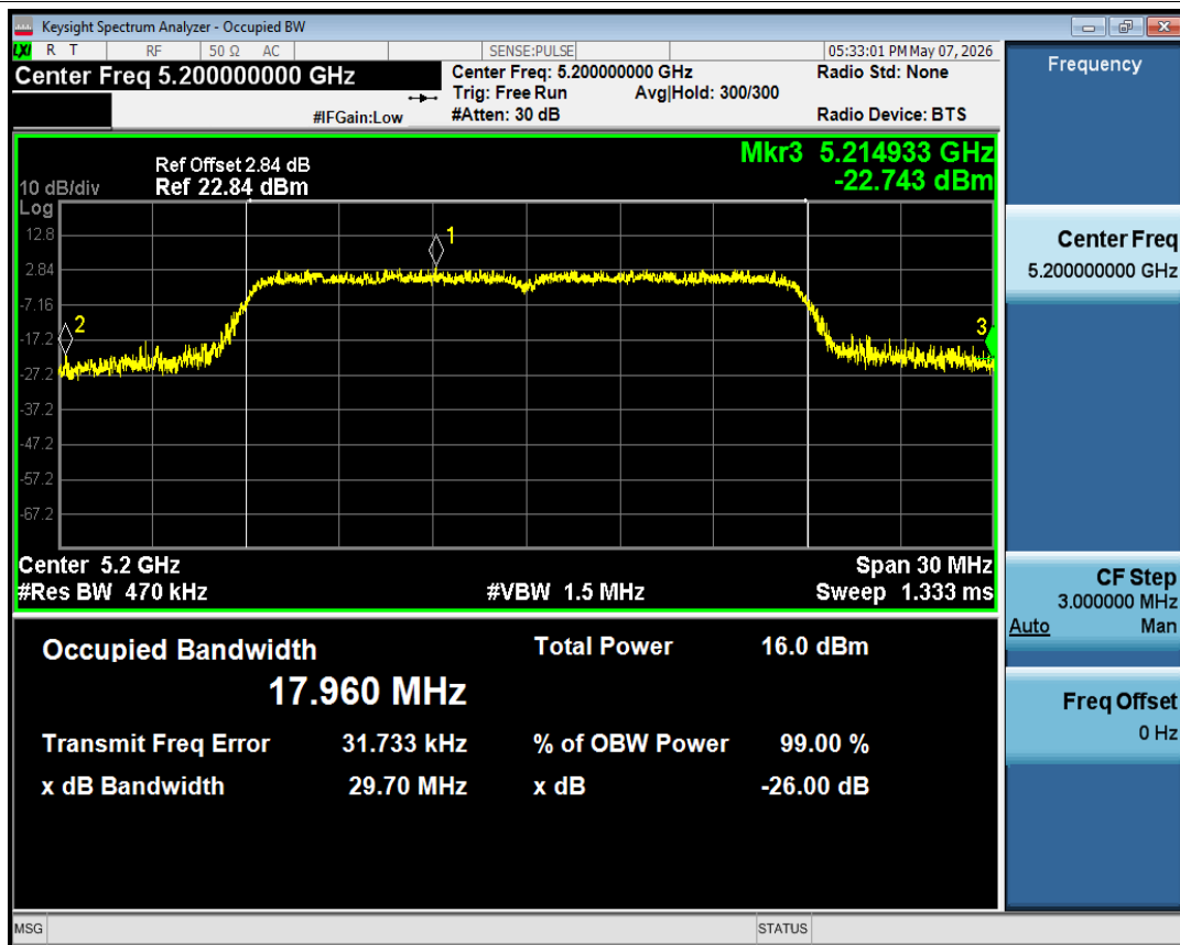
-26dB Bandwidth NVNT ax20 5200MHz Ant1
