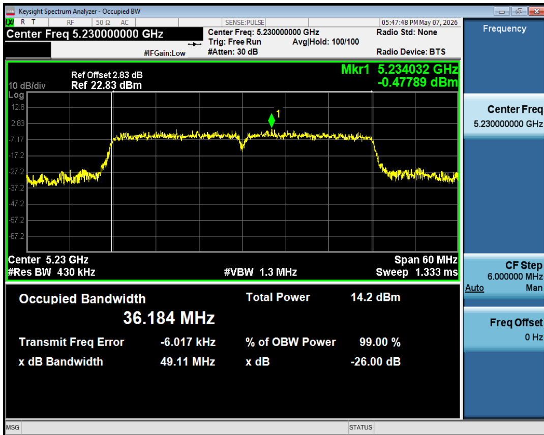
OBW NVNT ac40 5230MHz Ant1
