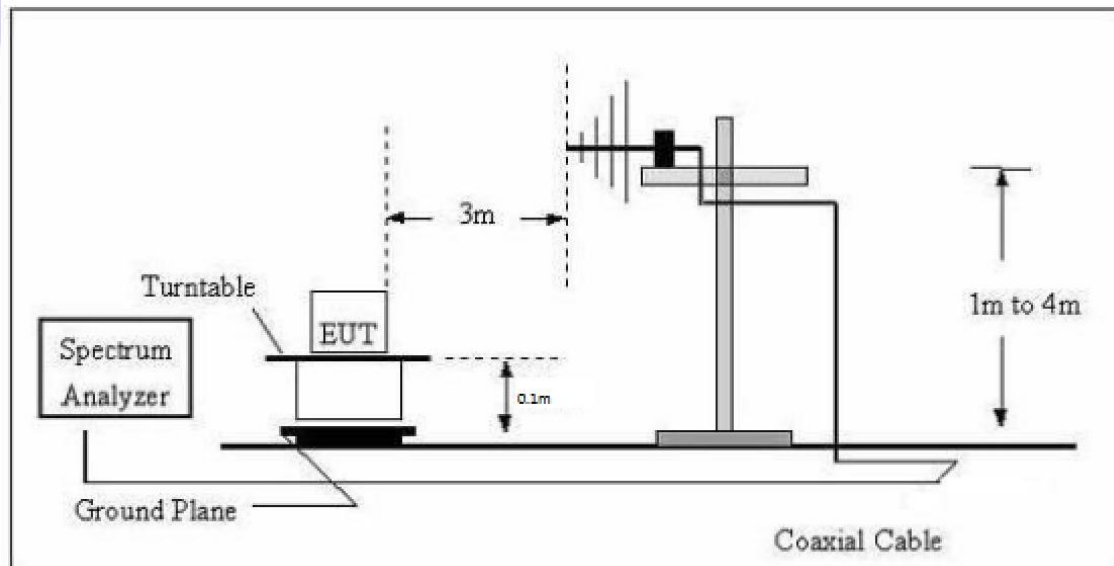
The test setup for emission measurement from 30 MHz to 1 GHz.
