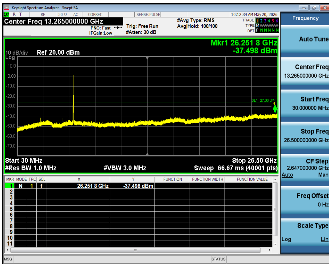
Tx. Spurious NVNT n20 5745MHz Ant1 Emission
