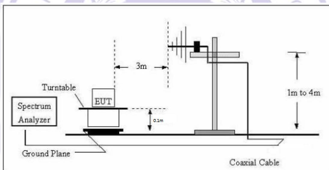
The test setup for emission measurement from 30 MHz to 1 GHz.
