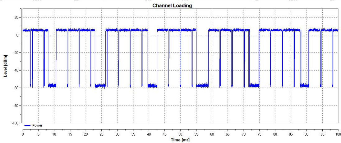
11AX40SISO_5670_Type0
