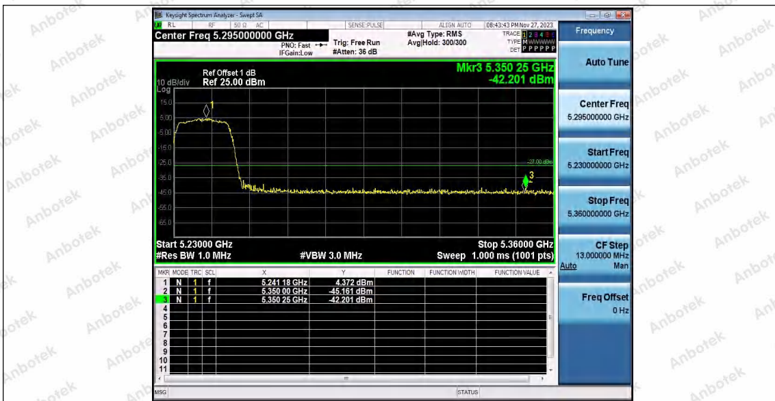
11N20SISO_Ant1_Low_5260
