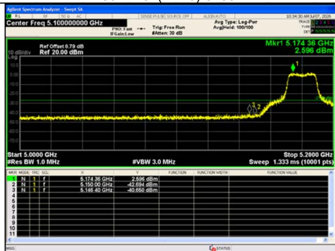
802.11ax(HE40)-5190
