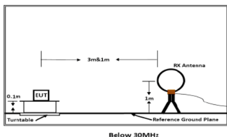
Figure 1. Below 30MHz
