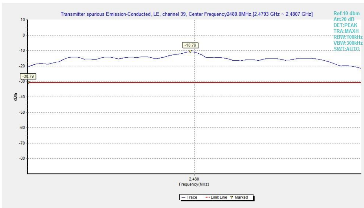
Fig.15 Conducted Spurious Emission (Ch39, Center Frequency)
