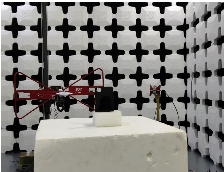
10. Radiated Emissions (Part 22/24/27/90) (30MHz-18GHz)
