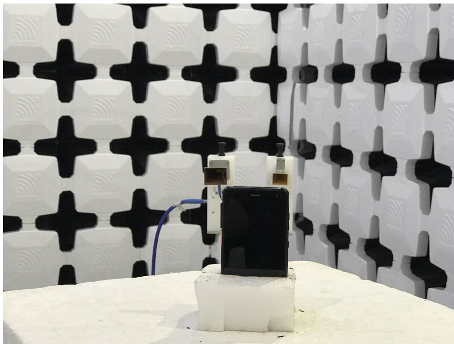
8. Radiated Emissions (Part 15C&E) (18-26.5GHz)
