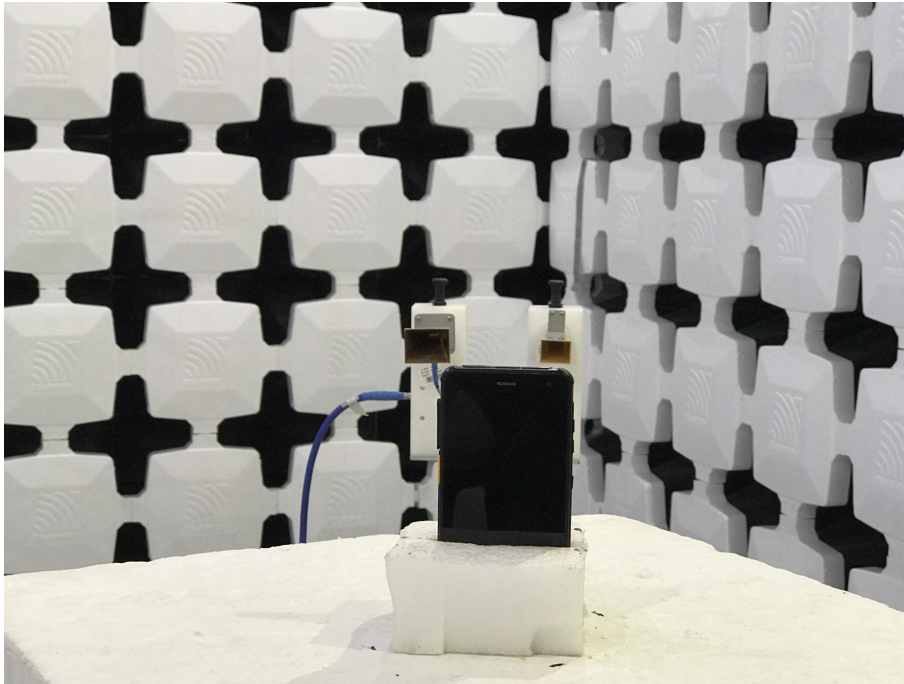
11. Radiated Emissions (Part 22/24/27/90) (18GHz-26.5GHz)
