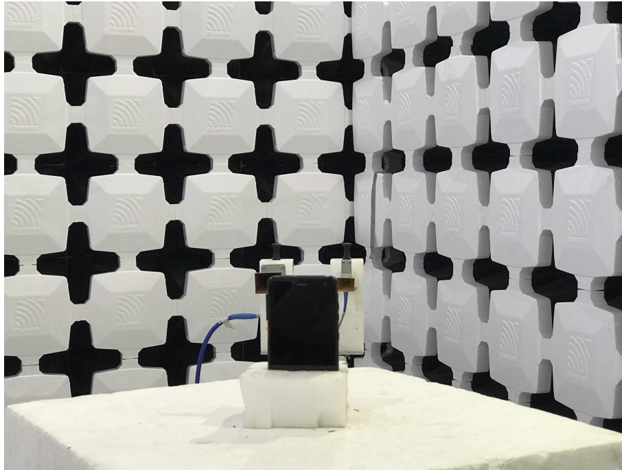
9. Radiated Emissions (Part 15C&E) (26.5-40GHz)
