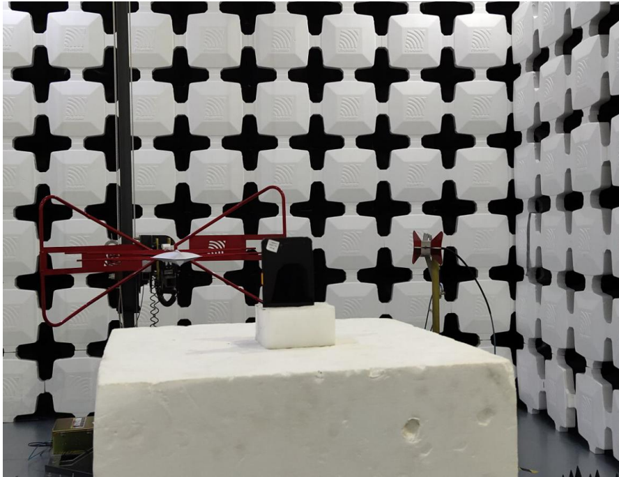
7. Radiated Emissions (Part 15C&E) (1-18GHz)
