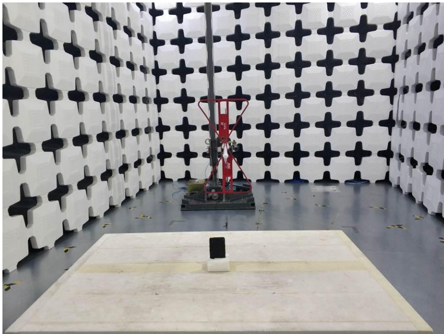
6. Radiated Emissions (Part 15C&E) 30MHz-1GHz)
