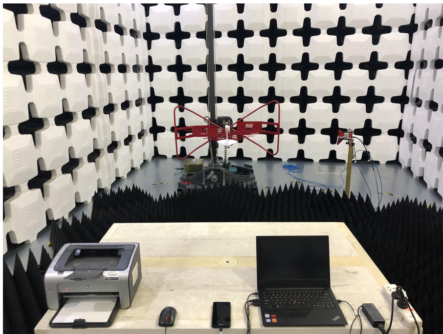
2. Radiated Emissions (Part 15B PC mode)( 1GHz-18GHz)
