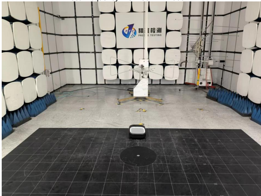
Test Frequency above 1G
